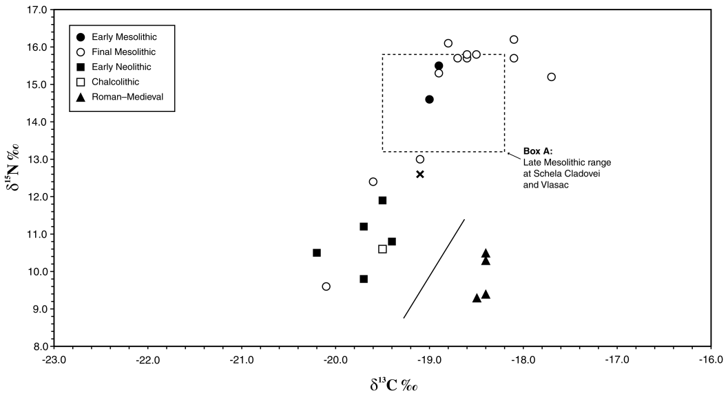
Figure 2 \delta^{13}\text{C} versus \delta^{15}\text{N} for 24 AMS ^{14}\text{C} -dated human skeletons from Lepenski Vir. The cross (x) represents an undated burial of Starčevo type.
