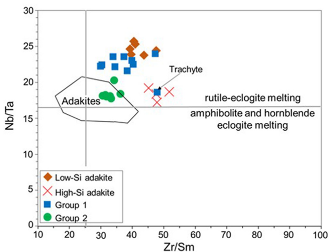
Fig. 12. Zr/Sm vs. Nb/Ta plot. The vertical line represents the average Zr/Sm value for primitive mantle (25.2; Sun and McDonough, 1989) and melting fields from Foley et al. (2002). The adakite field is from Condie (2005). Sample 4/626 from Group 2 is omitted (Nb/Ta = 40).
