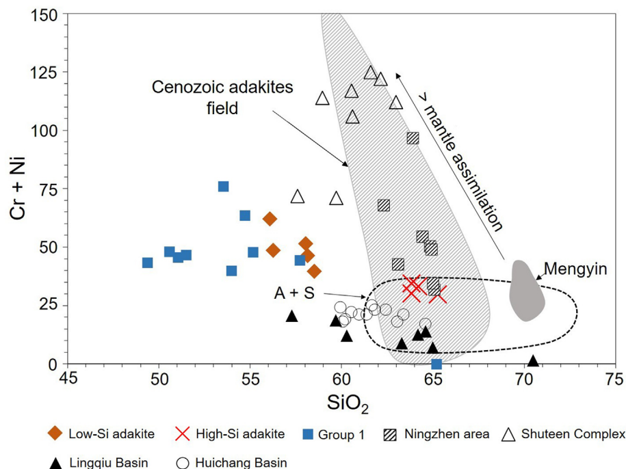
Fig. 11. SiO 2 wt. % vs. Cr + Ni (ppm) plot. Symbols and data sources are the same as in Fig. 9.
