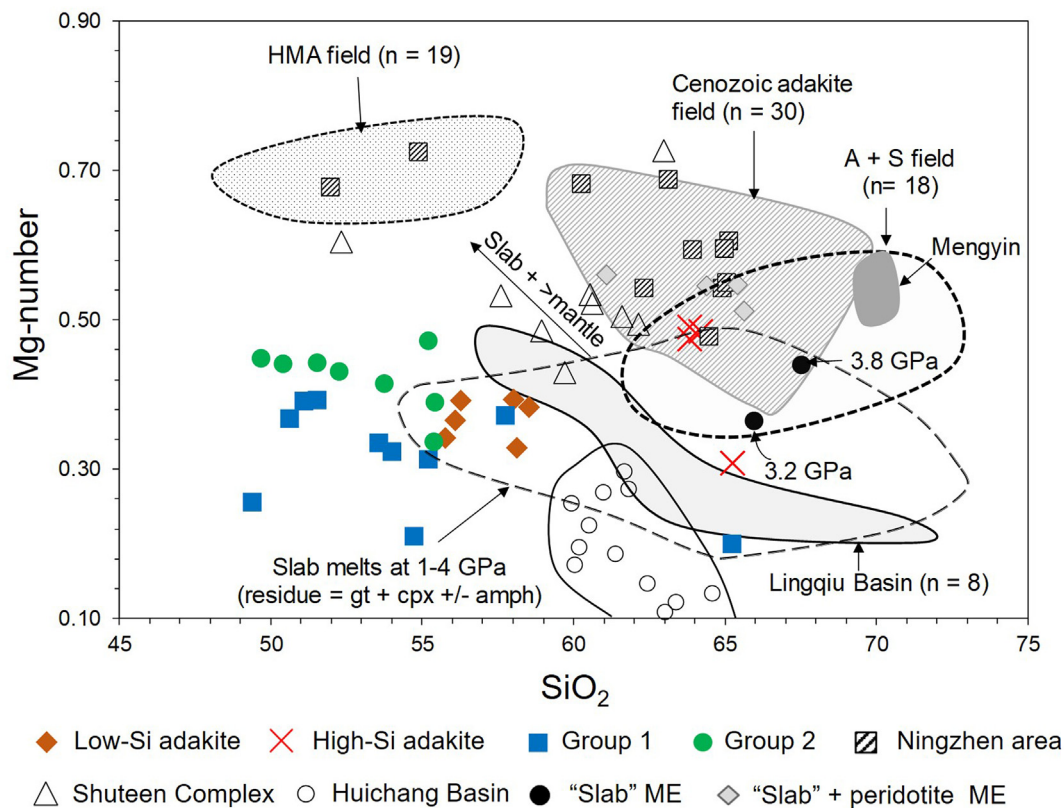
Fig. 9. \text{SiO}_2 wt. % vs. Mg-number (where Mg-number = {molar Mg/(Mg + Fe 3+ )}) plot. The “high-Mg andesite field” (HMA) represent oceanic eclogitic melts that interacted with the mantle wedge (Xu et al., 2000; Bryant et al., 2011). Shuteen Complex (Mongolia) adakites from Batkhishig et al. (2010) and Mengyin adakites (east China) from Wang et al. (2016). Ningzhen area (east China) samples were interpreted as delaminated lower crust which assimilated mantle (Xu et al., 2002). Huichang Basin, SE China (Xiong et al., 2003), and Lingqiu Basin, North China (Wang et al., 2006) samples represent melts of an underplated basaltic lower crust. The “A + S” field represent Awulale and Sanchakou (Xinjiang Tianshan region, China) adakitic rocks and are interpreted as a product of basaltic underplating at the base of the lower crust (Zhao et al., 2008). The “slab” melting and “slab” + peridotite (mantle) melting experiments (ME) and the 1–4 GPa “slab melts” field is based on data from Rapp et al. (1999, and references therein). The Cenozoic adakite field was generated from data within Aguillón-Robles et al. (2001) and Stern and Kilian (1996); Vizcaino Peninsula, Mexico; Lautaro; Viedma, Aguilera, Reclus; Mt Burney and Cook Island.
