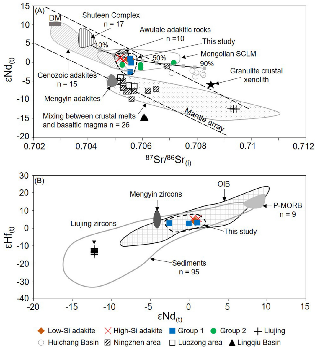
Fig. 13. (A) Plot of ^{87}Sr/^{86}Sr_{(i)} vs. \epsilon Nd(t) and (B) a plot of \epsilon Nd(t) vs. \epsilon Hf(t) . The mixing of crustal and basaltic melts field is from Chen et al. (2013). The Cenozoic adakites field is generated from: the Andean-Austral volcanic zone (Stern and Kilian, 1996; Lautaro, Viedma, Reclus and Mt. Burney); Cerro Pampa, South America (Kay et al., 1993); La Yeguada Volcanic Complex, Panama (Defant et al., 1991) and Vizcaino Peninsula, Mexico (Aguillón-Robles et al., 2001.). The P-MORB field generated from: Alexander Island, Antarctica; SW & NW Pacific crust and Venezuela (Barry et al., 2017 and references therein). Mongolian lithospheric melts field based on data from Sheldrick et al. (2018), and references therein). The depleted mantle (DM) is from Zindler and Hart (1986); mantle array is from Zhang et al. (2005); OIB field from Wang et al. (2016; and references therein) and sediment field from Vervoort et al. (1999) but excluded the Archean shales. The AFC modelling (equations from DePaolo, 1981) utilises a r value 0.5 and the starting composition used sample SH-18. The amount of F ranges from 1 to 0.1 and tick marks are in 10% intervals. The granulite contaminant (TB95–2.5) is from Barry et al. (2003) and isotopic values are age adjusted to 230 Ma. Other data from the same cited sources utilised for Fig. 9.
