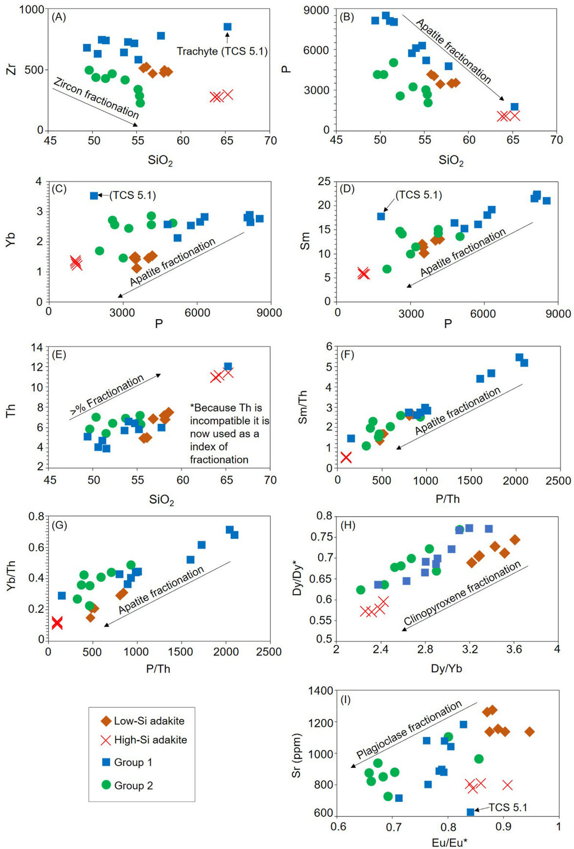
Fig. 7. Variations in major-element oxides (wt. %) and trace elements (ppm) for the low-Si adakites, high-Si adakites, Group 1 and 2 samples. Where \frac{Dy}{Dy^*} = \frac{Dy_n}{La_n^{0.13}Yb_n^{0.13}} (Davidson et al., 2012). The chondrite normalisation values are from Sun and McDonough (1989).
