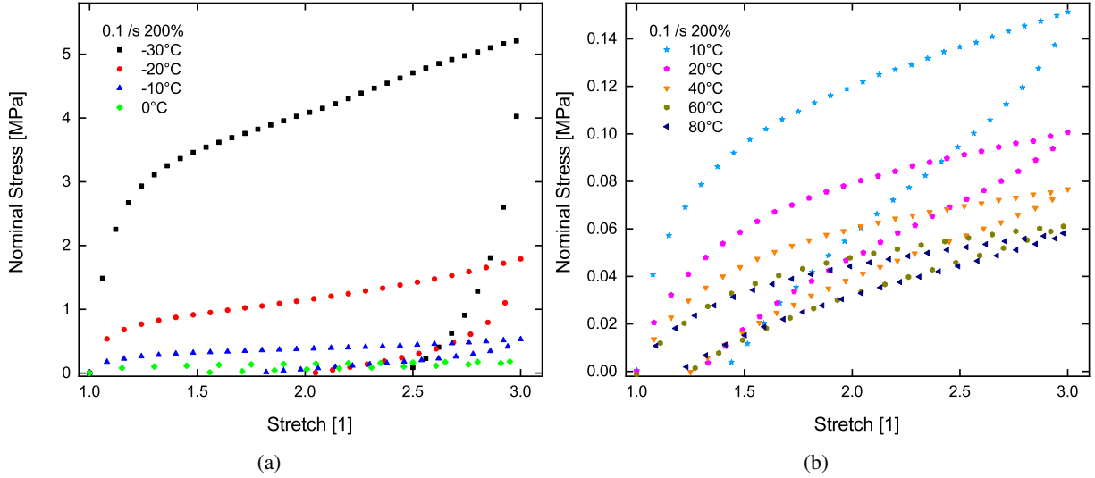
Figure 7: Temperature-dependent stress response under a wide range of temperature where experiments are conducted at 200% strain and 0.1 /s strain rate, (a) below 0°C, (b) above 0°C. All results clearly reveal that the temperature field has a major role in changing mechanical stress responses of the VHB polymer.
