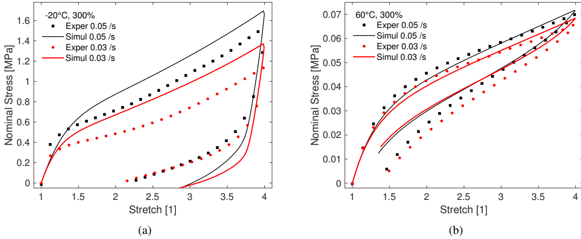
Figure 19: Thermo-viscoelastic model validation from 0.03 /s to 0.05 /s strain rates of 300% strain: (a) -20°C, (b) 60°C.
