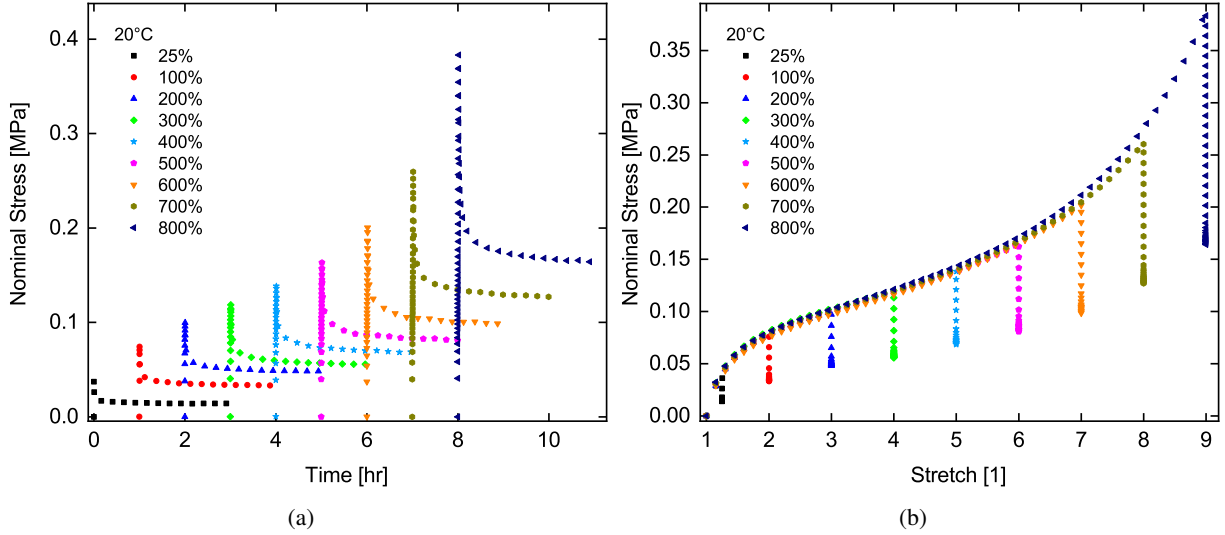
Figure 9: Single-step relaxation test results from 25% to 800% strains. (a) Stress histories with respect to relaxation times, (b) Stress-strain curves depicting the amount of stress relaxations during the holding times
