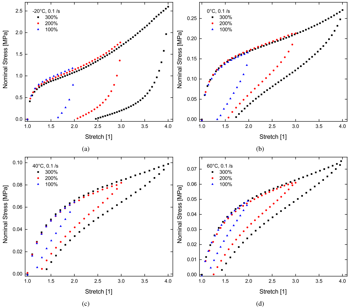
Figure 5: Stress response and cyclic dissipation of three strain levels (100%, 200%, and 300%) with respect to temperature variations at a fixed strain rate of 0.1 /s, (a) -20°C, (b) 0°C, (c) 40°C, (d) 60°C. These results demonstrate that the VHB 4905 becomes less dissipative with an increasing positive temperature
