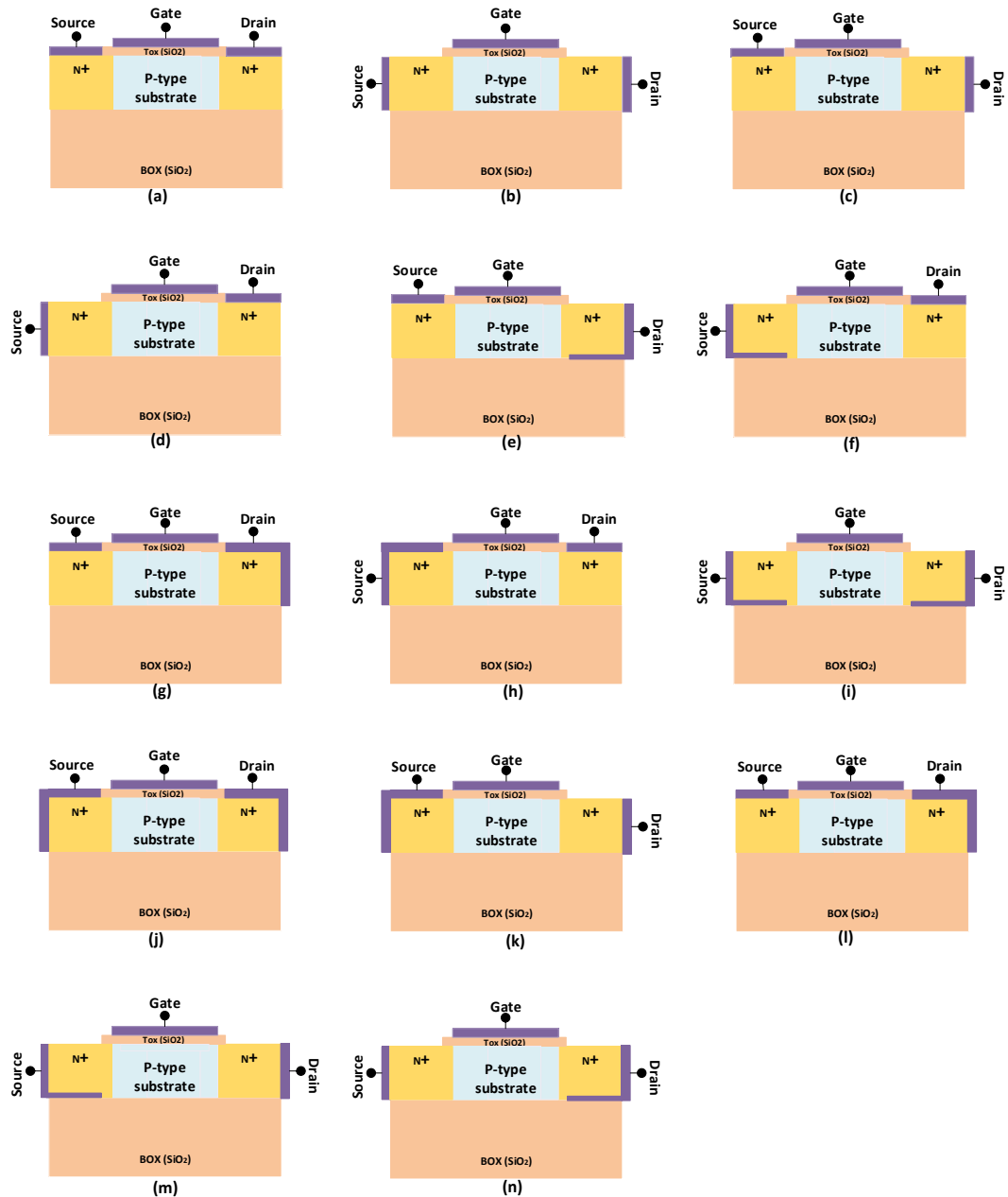
Fig. 1. Different source and drain electrodes geometry considered in this research.
