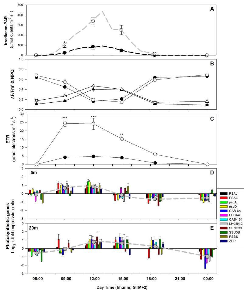
Figure 1. Daily cycle of PAR irradiance (A), quantum yield of PSII (circles in B), non-photochemical quenching downregulation (triangles in B) and electron transport rates (C) of shallow (white symbols) and deep (black symbols) P. oceanica plants; and daily variation of mRNA expression of photosynthesis-related genes at 5 m (D) and 20 m (E) depth. Relative expression levels at given time points are calculated over their daily average expression. Dashed lines represent the average expression level of all analyzed genes. Asterisks indicate significant differences among shallow and deep plants at a given sampling time. ** p < 0.01 ; *** p < 0.001 .
