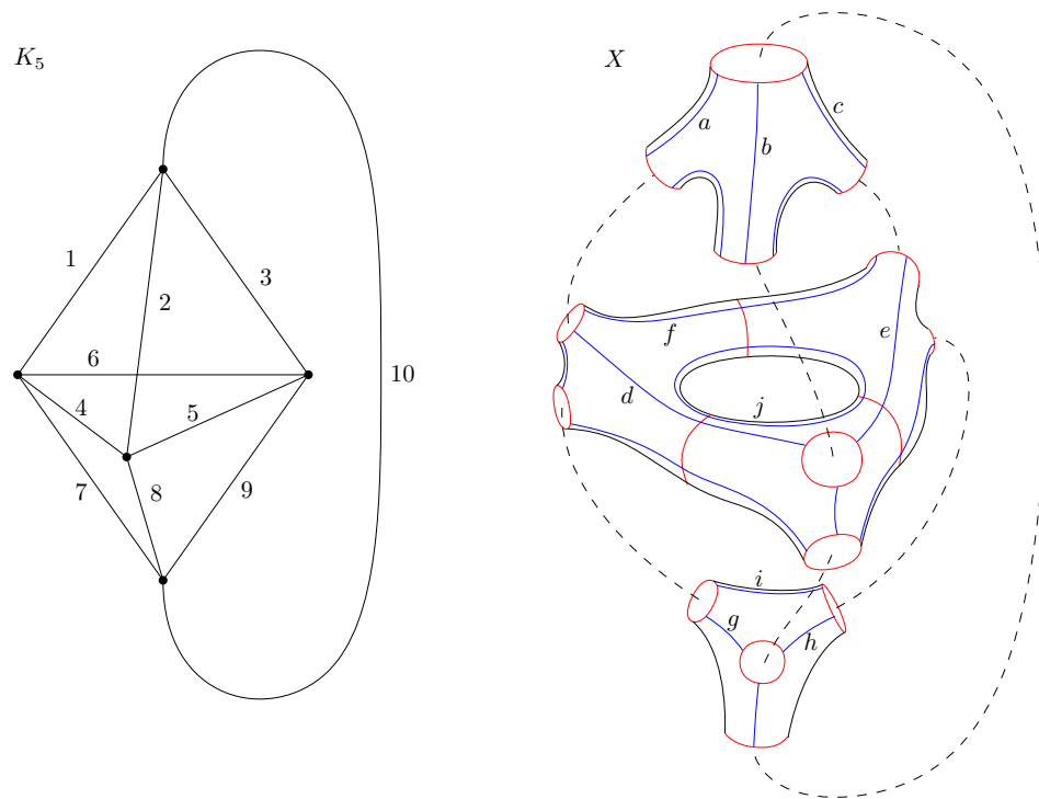
Figure 1: An embedding of K_5 in \mathbb{R}^3 and the corresponding gluing of tetrahedral blocks.
