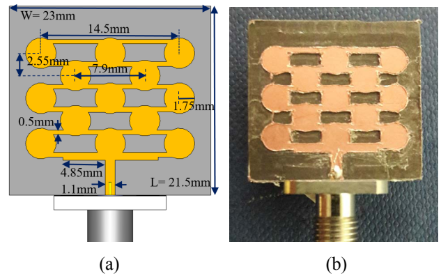
Fig. 1. The geometry of the proposed grid antenna array for 5G; (a) simulated model with the optimized dimensions, (b) fabricated prototype.
