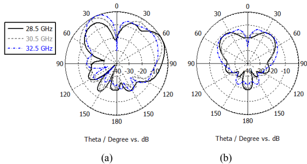
Fig. 3. Numerically computed normalized radiation pattern of the proposed antenna grid array at three distinct frequencies: (a) E-plane cut at \phi = 90^\circ , (b) H-plane cut at \phi = 0^\circ .
