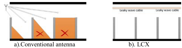
FIGURE 3. Conventional antenna creates shadow zones while LCX cable covers wider area. a). Conventional antenna. b). LCX.
