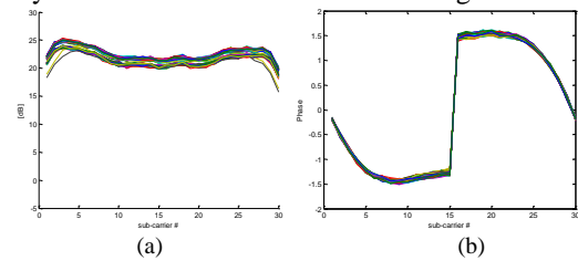
(a). The channel information data recorded using LWC (b). The sanitized phase information obtained during the experiment
