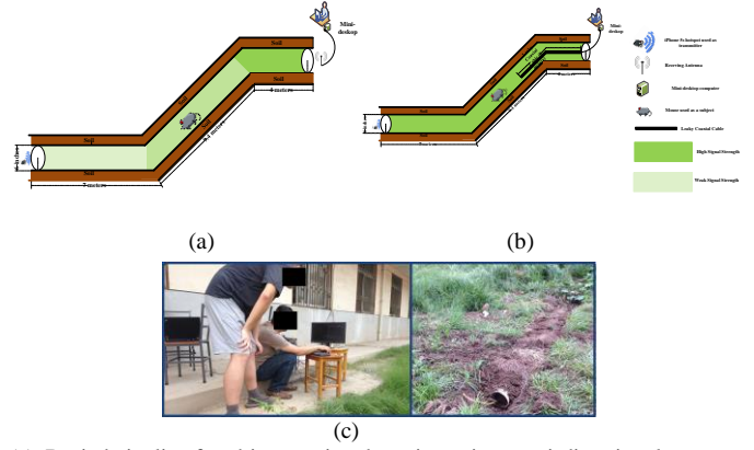
(a). Buried pipeline for object motion detection using omni-directional antenna. (b). Buried pipeline for object motion detection using LWC.
