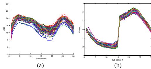
(a). Variances of CFR data due to subject motion. (b). Variation in phase information.
