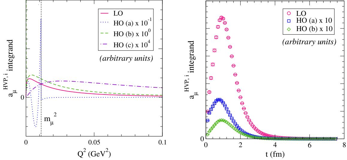
FIG. 3. Left: integrands of Eqs. (A1) (blue dots), (A6) (green dashes), and (A13) (purple dot-dashes) obtained from the N = 2 + 1 + 1 Mellin-Barnes approximant for \hat{\Pi}(Q^2) given in Ref. [25], which employs preliminary moments of R_\gamma(s) provided by Keshavarzi et al. [16]. The leading-order integrand is also shown as a solid magenta line for comparison. Right: integrands of Eqs. (A3) (blue squares) and (A11) (green diamonds) obtained from the parameterization of R_\gamma(s) provided by Jegerlehner in his public alphaQED FORTRAN package [30]. The leading-order integrand is also shown as magenta circles for comparison.
