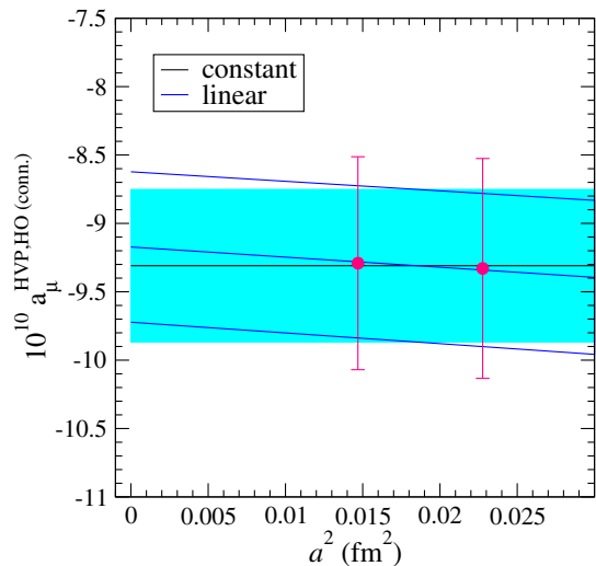
FIG. 5. Continuum extrapolation of O(\alpha^3) quark-connected contribution to a_\mu^{\text{HVP}} . The filled cyan band shows the result of our preferred constant fit, while the solid blue lines show the result of a linear fit to Eq. (3.3) with the slope c_{a^2} constrained with a Gaussian prior 0 \pm 1 .
