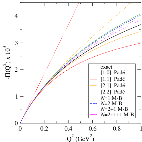
FIG. 4. First four Padé approximants (“[1,0]–[2,2] Padé”) and Mellin-Barnes approximants (“ N = 1 - N = 2 + 1 + 1 M-B”) of the renormalized vacuum polarization function calculated from the moments of R_\gamma(s) analysis of Keshavarzi et al. [16]. The exact result is shown as a solid black line for comparison [34].
