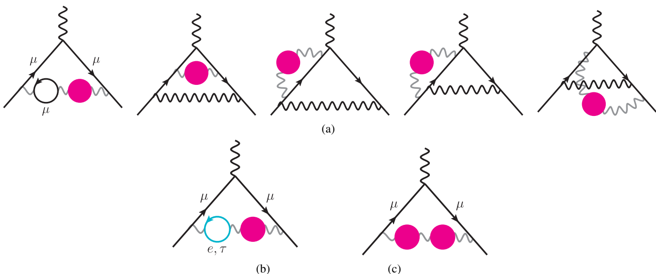
FIG. 2. Higher-order hadronic-vacuum-polarization contributions to g_\mu - 2 . For contribution (a), diagrams that are reflections across the vertical axis through the center and diagrams in which the tree and corrected photon propagators are interchanged are not shown.
