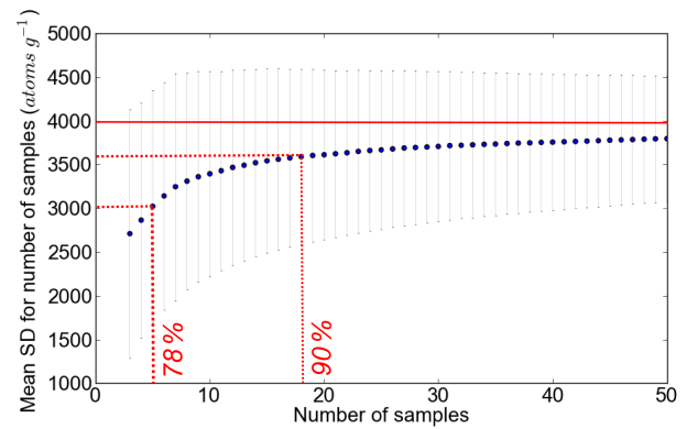
Figure 12. Number of ^{10}\text{Be} samples required to capture the natural concentration variability of the Ganga River. Approximately 18 samples are required to be within 10 % of the true standard deviation (or variability) of the system. Blue dots represent the mean standard deviation of 100 populations of concentrations for a given sample group size (between 3 and 50). Error bars represent the standard deviation of the mean standard deviation of those 100 populations per sample group size. The solid horizontal red line represents the mean standard deviation value that the sample group sizes converge towards (4000 atoms \text{g}^{-1} ). The two dashed red lines represent the number of samples required to be within 10 % of the true standard deviation (labelled 90 %) and the standard deviation expected from a set of five samples (labelled 78 %).
