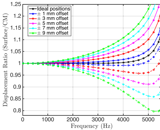
FIG. 10. Calibration errors resulting from the bulk elastic deformation of the test mass induced by calibration forces. Results of finite element analysis using COMSOL Multiphysics ® for Pcal beams displaced symmetrically away from (solid lines) and toward (dashed lines) the center of the test mass from their ideal locations. The data are the ratio of the motion of the surface, as sensed by the main interferometer beam that has a Gaussian spatial profile, divided by the center of mass motion.
