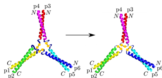
Figure 3. If the designed dimer peptides preferentially interact, when allowed to rearrange, the disulfide bonds should switch to being between the desired pairs, with the species present in the system moving from p6–p1, p3–p2, and p4–p5 to p1–p2, p3–p4, and p5–p6.
