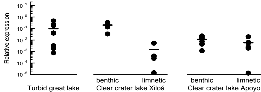
Figure 3. Distribution of estimated proportion of vitamin A2-derived chromophore usage in Midas cichlids from the turbid great lake Nicaragua and two clear water crater lakes (a). Estimates of A2-derived usage for the long-green spectral class were not included due to the confounded effect of opsin coexpression. cyp27c1 expression relative to the geometric mean of two housekeeping genes ( Idh2 and inp2 ) in the same crater lakes and the turbid great lake Managua (b). Horizontal lines are the mean for each group. Bonferroni corrected pair-wised comparisons are reported in supplementary table S2, Supplementary Materials online.
