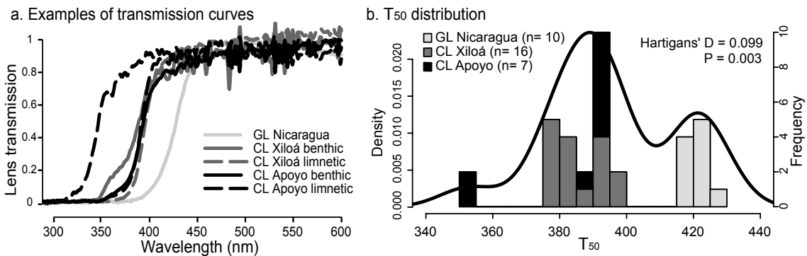
Figure 4. Lens transmittance grouped into different categories. Example of these are shown in (a). Histogram depicting the frequency of lens transmittance cut-offs ( T_{50} ) of lab-reared Midas cichlids (b). Over-imposed is a density kernel showing the bimodal distribution of T_{50} .
