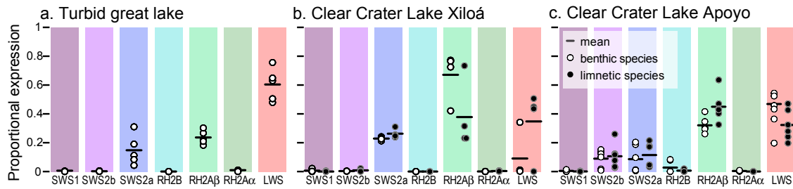
Figure 5. Proportion of the total opsin expression comprised by each of the different opsin genes in wild-caught Midas cichlids from a turbid great lake (a), and two clear crater lakes (b, c). Means are shown as horizontal bars. Black circles represent expression in specimens of the limnetic ecomorph, white circles denote expression in specimens of the benthic species.
