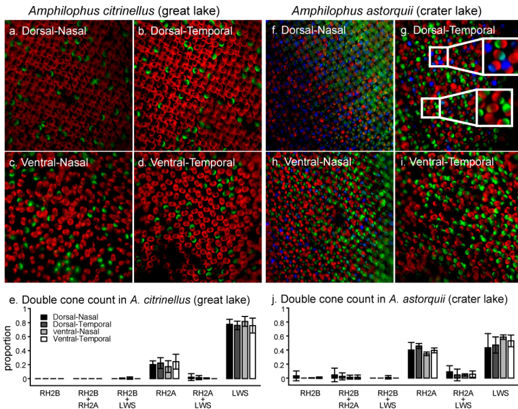
Figure 6. Triple fluorescent in situ hybridization staining of the retinas of two Midas cichlid species, one from a turbid great lake (a-e) and one from a clear crater lake (f-j) across four quadrants of the retina. Coexpression is common in specimens from both lakes, but the frequency is higher in specimens from the clear crater lake (f-j). Details in (g) show examples of coexpression of LWS and RH2Aβ (upper box) and RH2B and RH2Aβ (lower box).
