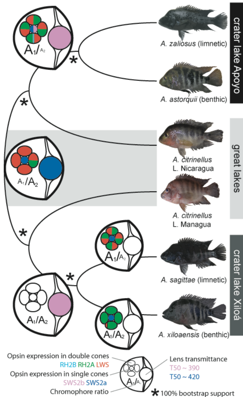
Figure 7. The visual system of Midas cichlids evolved in parallel in the two clear crater lakes Apoyo and Xiloá after their colonization from the turbid great lakes Nicaragua and Managua, respectively. Phenotypic changes in opsin expression, chromophore usage and lens transmittance are mapped on a phylogenetic reconstruction modified from Kautt et al. (2016a). In fish from both crater lakes, lenses became more transmissive and expression of RH2A increased and that of LWS decreased. In all crater lake species, except for A. xiloaensis , chromophore usage changed from mainly A2 to mainly A1.
