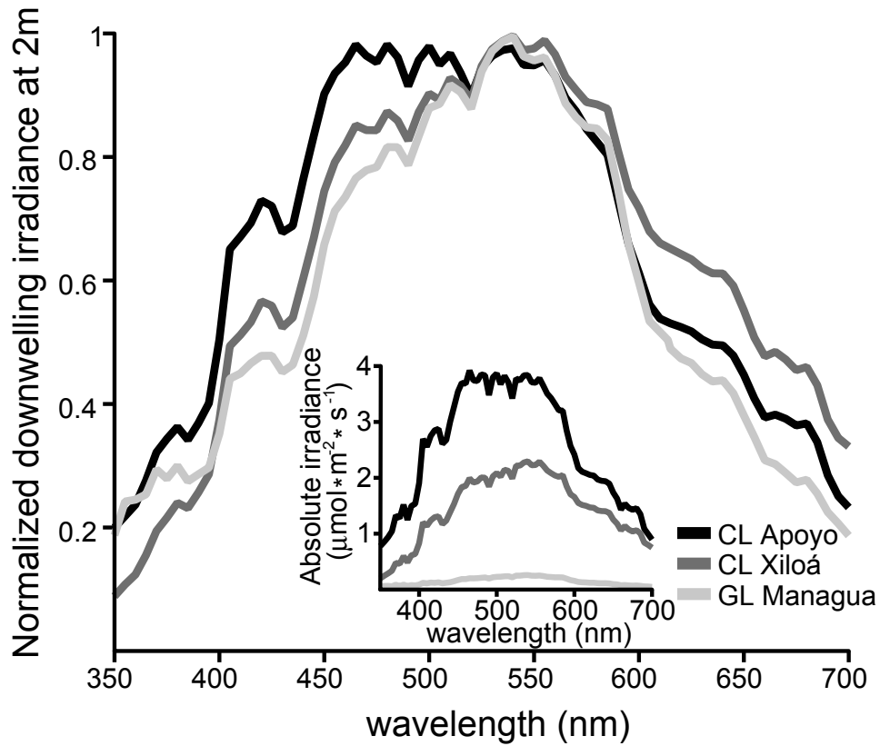
Figure 1. Difference in the photic environment of a great lake and the crater lakes.
