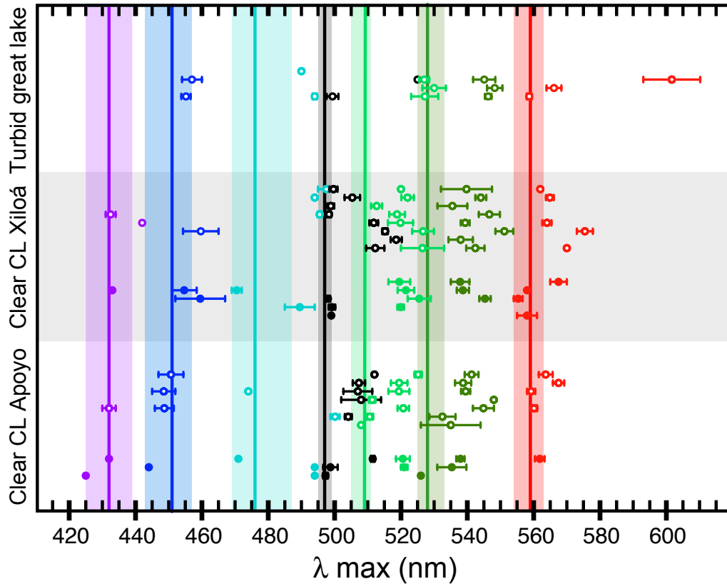
Figure 2. Individual level peaks of maximum absorbance ( \lambda_{\max} \pm \text{SE} ) of visual pigments determined by microspectrophotometry from wild-caught Midas cichlids from a turbid great lake and to clear crater lakes. Unfilled symbols correspond to specimens of the benthic ecomorph within each lake, whereas filled symbols correspond to limnetic specimens. Visual pigments were assigned to different spectral classes (indicated by the vertical lines of different colors) based on their estimated pure A1 peak of maximum absorbance ( \lambda_{A1} ). The ranges of estimated \lambda_{A1} are shown as shaded areas of the same color. From left to right, these spectral classes correspond to the violet, blue, blue-green, rod, green (short), green (long), and red previously identified in African cichlids (Carleton et al. 2009). The grey shading separates samples from the different lakes.
