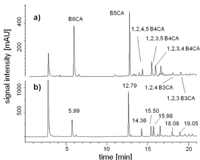
Figure 2: Chromatograms for BPCA Separation. Shown are the black carbon reference materials "chernozem" (a) and "grass char" (b). Baseline separation is achieved for all the BPCA target compounds (B6CA; B5CA; 1,2,4,5-, 1,2,3,5-, 1,2,3,4-B4CA; 1,2,4-, 1,2,3-B3CA) 42 . Information on the black carbon reference materials is available from the University of Zurich ( http://www.geo.uzh.ch/en/units/physische-geographie-boden-biogeographie/services/black-carbon-reference-materials ). This figure was modified from Wiedemeier et al. 2013 42 and is reprinted with permission from Elsevier. Please click here to view a larger version of this figure.
