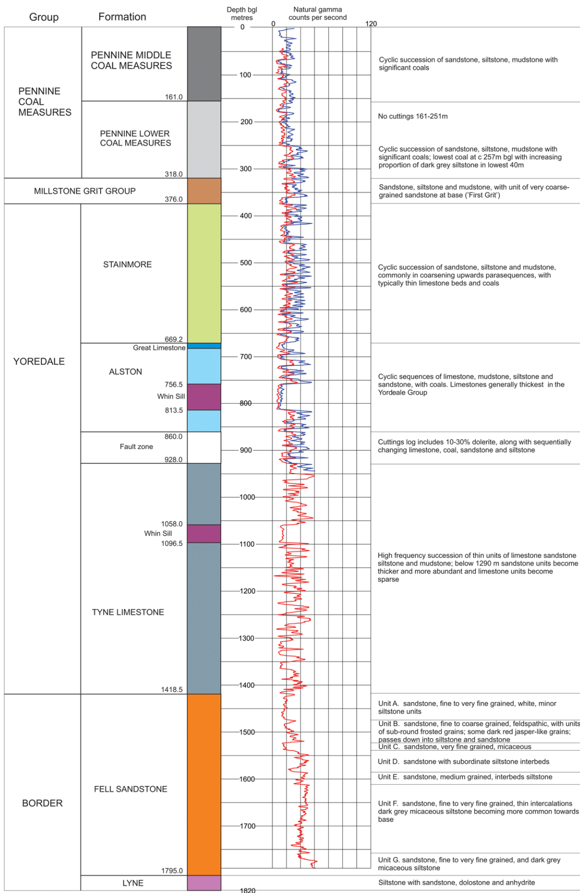
Fig. 3. Summary interpreted geological log for the Science Central Borehole, with natural gamma-ray logs that were used to assist interpretation of cuttings.
