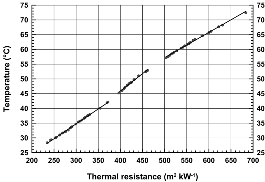
Fig. 5. Bullard thermal resistance plot calculated for depths below 500 m in the Science Central Borehole. Linear regression has been applied to sections of the plot corresponding to the upper, middle and lower sections of the borehole.
