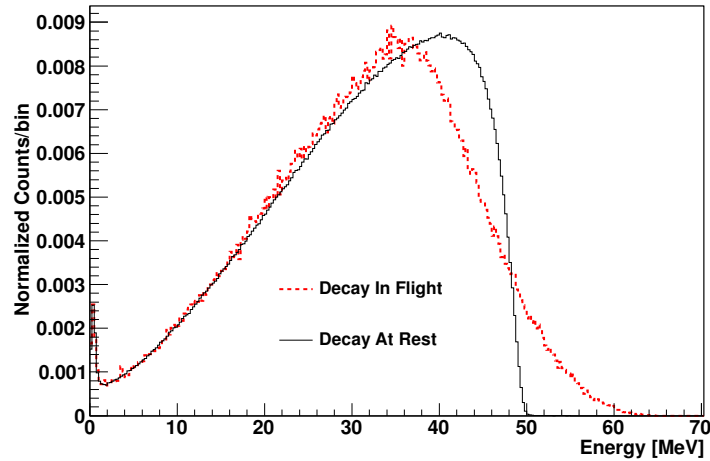
Figure 10. \pi^+ \rightarrow \mu^+ \rightarrow e^+ energy spectra. Red (dashed line): Simulated \mu DIF events. Black (solid line): Decay-at-rest events.
