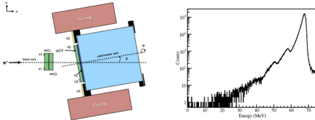
Figure 9. Left: Schematic of the calorimeter lineshape measurement.[13] Right: Energy spectrum in NaI and CsI at 0°[14].
