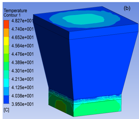
Figure 3 Comparison of average temperature between prediction and measurement based on the new model as well as temperature contour on outside surfaces of the model, (a) average temperature versus incidence, (b) temperature on outside surfaces at 0° incidence
