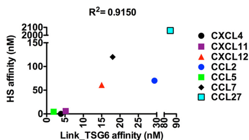
FIGURE 3. Correlation between chemokine affinity for Link_TSG6 and HS. Kinetic affinity estimates for each chemokine binding to immobilized HS (56, 57) or Link_TSG6 are plotted, as calculated using SPR. Data shown are from individual measurements representative of two independent experiments. CXCL8 is excluded from this figure as previous studies did not enable evaluation of a robust affinity estimate for the CXCL8/HS interaction (57).
