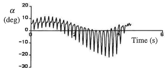
Figure 10 : Angle of Attack of Hibrom Inboard Blade Station During Pop-up (85kts)
