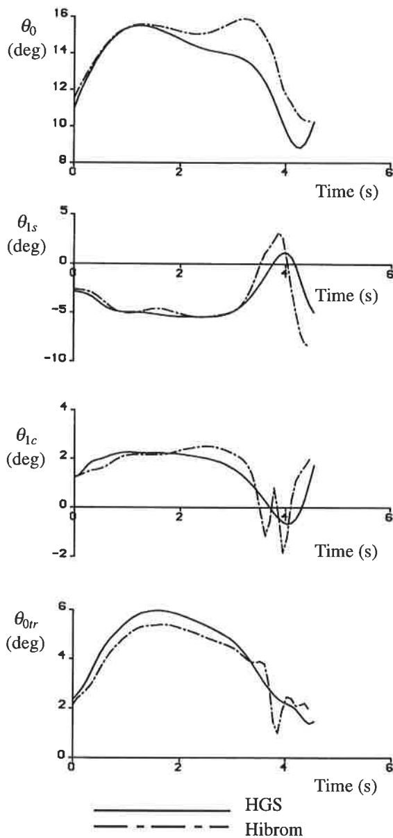
Figure 8 : Inverse Simulation of a Pop-up Manoeuvre ( s = 200m , h=25m , V_f = 85kts ) with Data for Westland Lynx Helicopter
