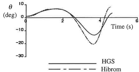
Figure 9 : Fuselage Pitch Angle During Pop-up (85kts) Manoeuvre
