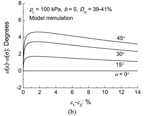
Figure 2. Comparison between the observed and model predicted non-coaxial sand behaviour in undrained torsional shear tests (data from Yoshimine et al. 1998).
