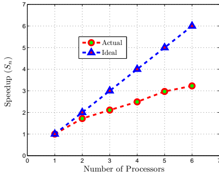
(b) Speedup
