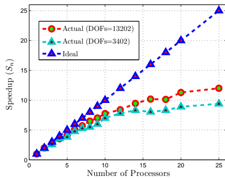
(c) Speedup
