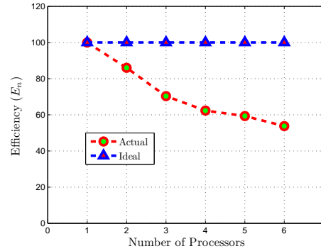
(c) Efficiency
