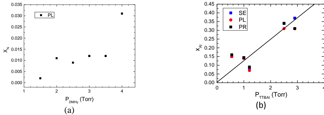
Figure 2. (a) N mole fraction in \text{GaAs}_{1-x}\text{N}_x as a function of DMHy gas precursor flux at a growth rate of 0.5 \mu\text{m/h} and a substrate temperature of 500 ^\circ\text{C} . (b) Al mole fraction in \text{Al}_x\text{Ga}_{1-x}\text{As} as a function of TTBAI gas precursor flux at a growth rate of 0.3 \mu\text{m/h} and a substrate temperature of 560 ^\circ\text{C} .
