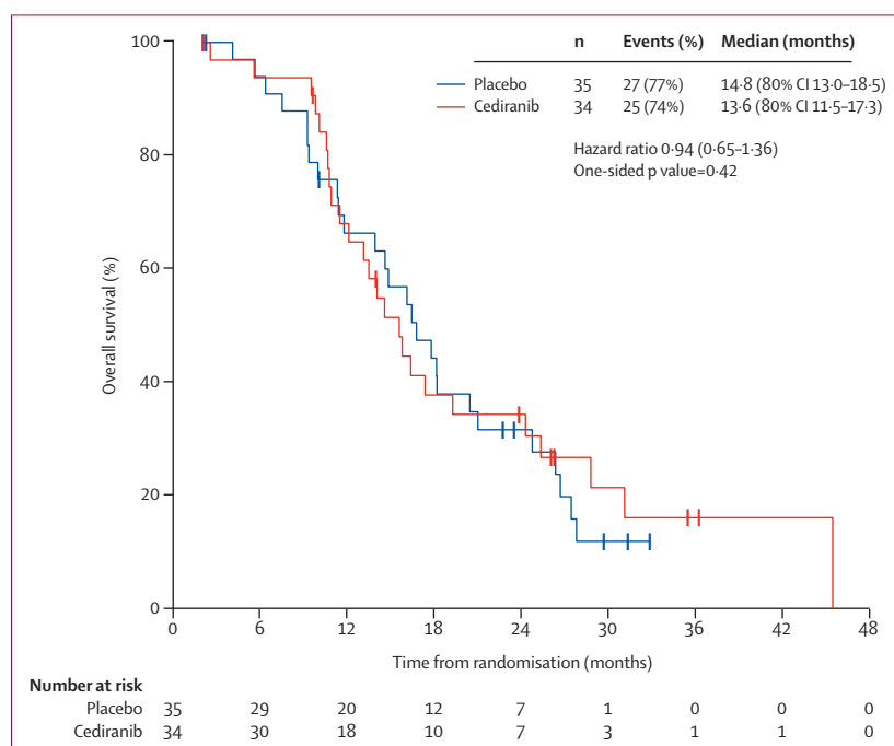
Figure 3: Overall survival
