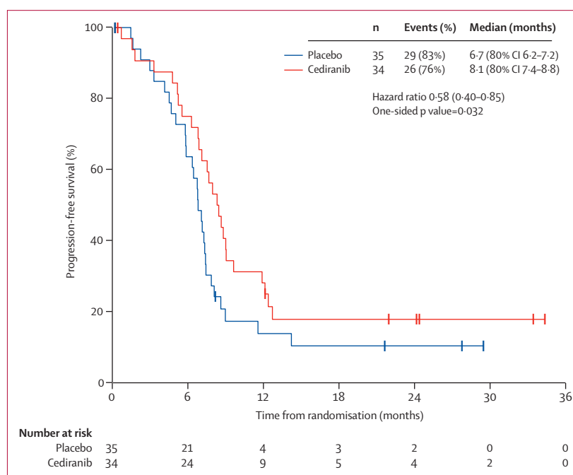
Figure 2: Progression-free survival
