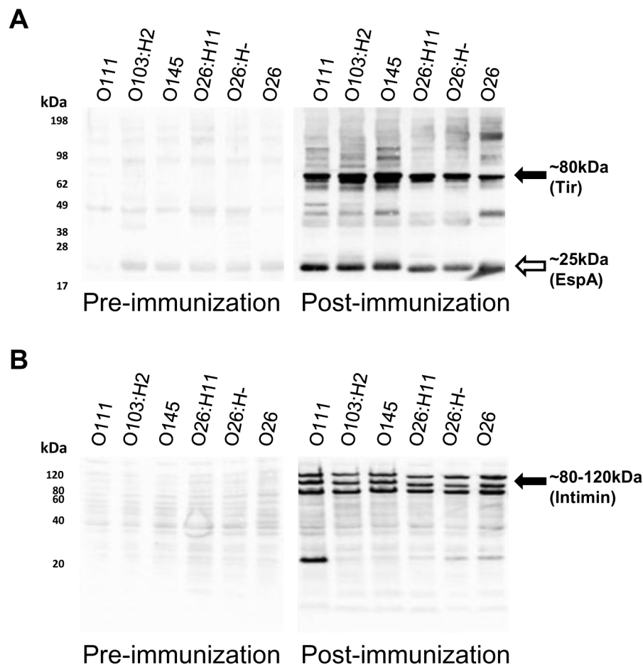
Fig 5. Cross-reactivity of vaccine-induced antibodies with secreted and whole cell antigen preparations from non-O157 EHEC serotypes. Representative western blot of (A) secreted protein preparations and (B) whole cell preparations from EHEC serotypes O111, O103:H2, O145, O26:H11, O26:H- and O26 with serum collected from a calf collected 2 days prior to first immunization (Pre-immunization) and 6 days after the final immunization (Post-immunization) with recombinant EspA, intimin and Tir. Bound IgG1 was visualized by chemiluminescence. The putative identities of EspA, Tir and intimin-reactive bands are indicated in brackets.
