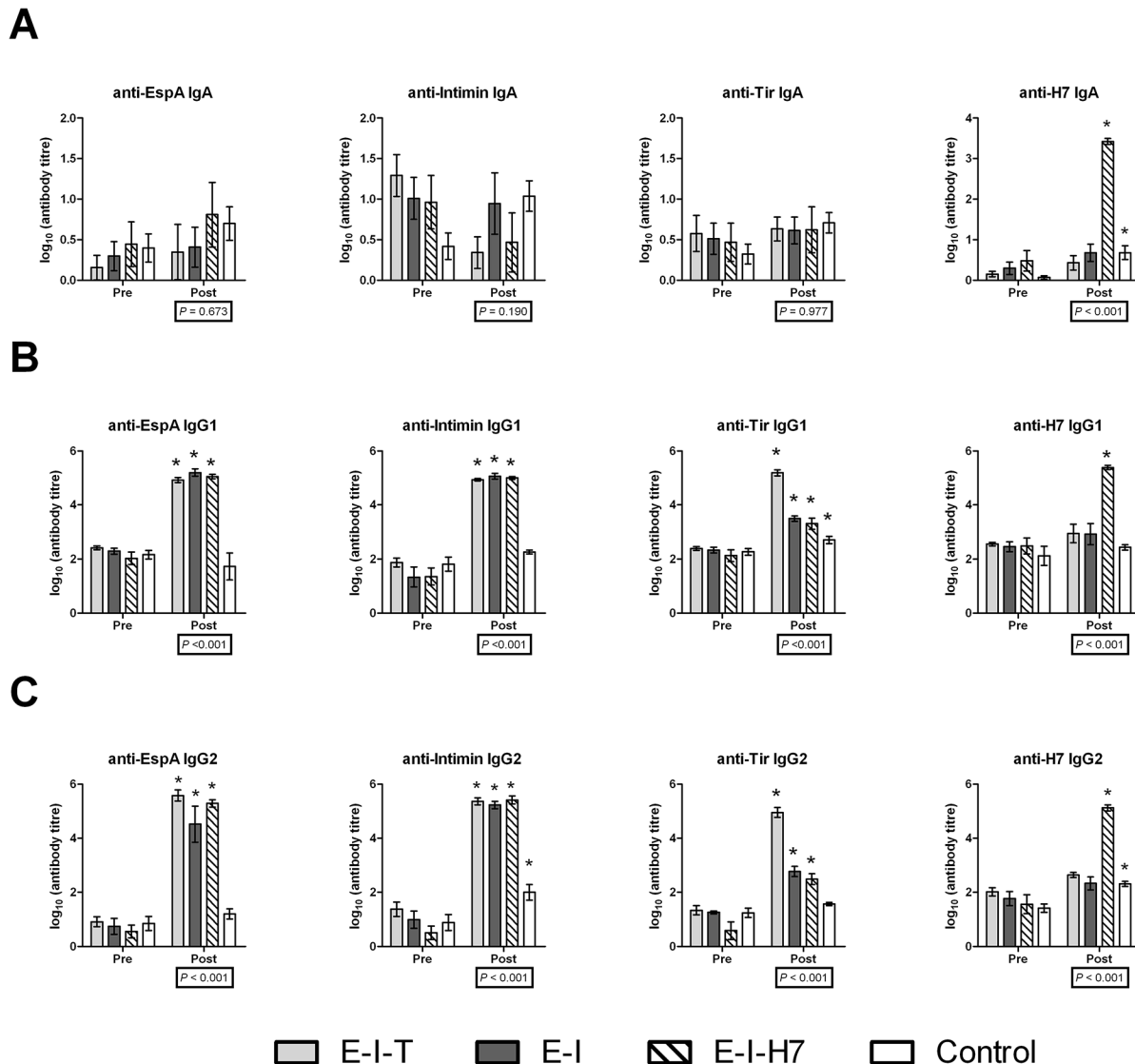
Fig 4. Serum antibody titres of different immunization groups. Mean titres of (A) IgA, (B) IgG1 and (C) IgG2 of EspA-, Intimin-, Tir- and H7 flagellin (H7)-specific antibodies within the serum of calves 2 days prior to the first immunization (Pre) and 6 days after the final immunization (Post) with either EspA, intimin and Tir (E-I-T), EspA and intimin (E-I), EspA, intimin and H7 flagellin (E-I-H7), or adjuvant alone (Control). Each bar represents the mean (on log 10 scale) and corresponding error bar shows the standard error of mean. Overall statistical significance of immunization group for each antibody titre post-immunization was assessed using a linear mixed model and indicated by a p -value below each graph. The mean difference in titres between pre- and post-immunization for each immunization group was investigated using a linear mixed model, and statistically significant (adjusted for false discovery rate, p F < 0.05) changes are indicated by an asterisk (*).
