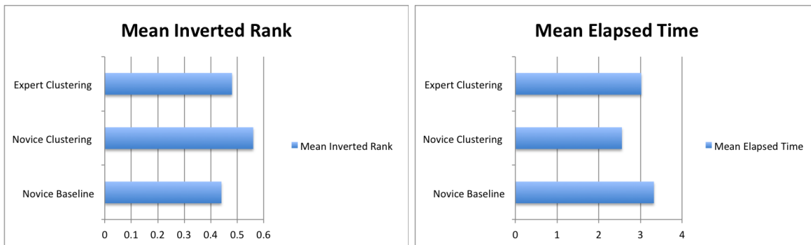
Figure 5: Official TRECVID KIS results
