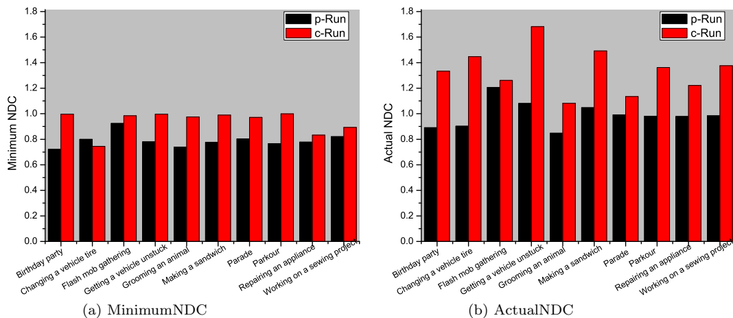
Figure 6: MinimumNDC and ActualNDC for each event. Note lower Actual NDC means better performance.
