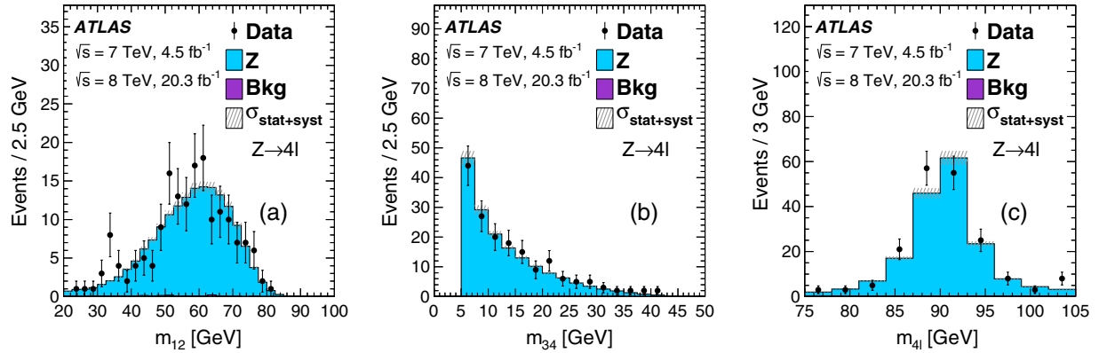
FIG. 2 (color online). Data and MC invariant mass distributions of (a) the leading lepton pair, m_{l2} , (b) the subleading lepton pair, m_{34} , and (c) the four-lepton system, m_{4\ell} . All selections are applied except in (c) there is no m_{4\ell} requirement. The background contributes < 1\% of the total expected signal (invisible in the plots).
