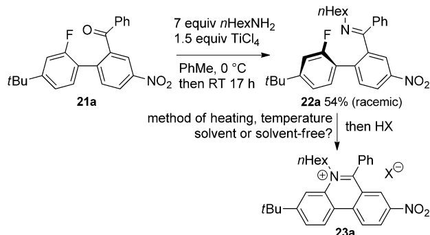
Scheme 5. Method development for construction of the B-ring.
