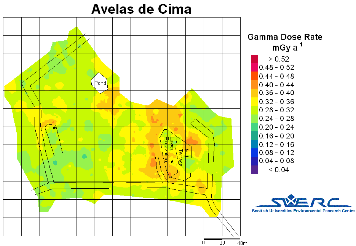
Figure 2: Dose rate distribution at Avelas de Cima.
