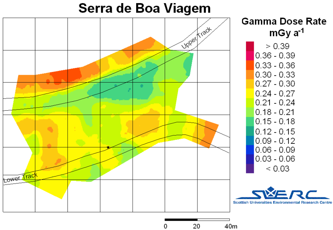
Figure 1: Dose rate distribution at Serra de Boa Viagem.
