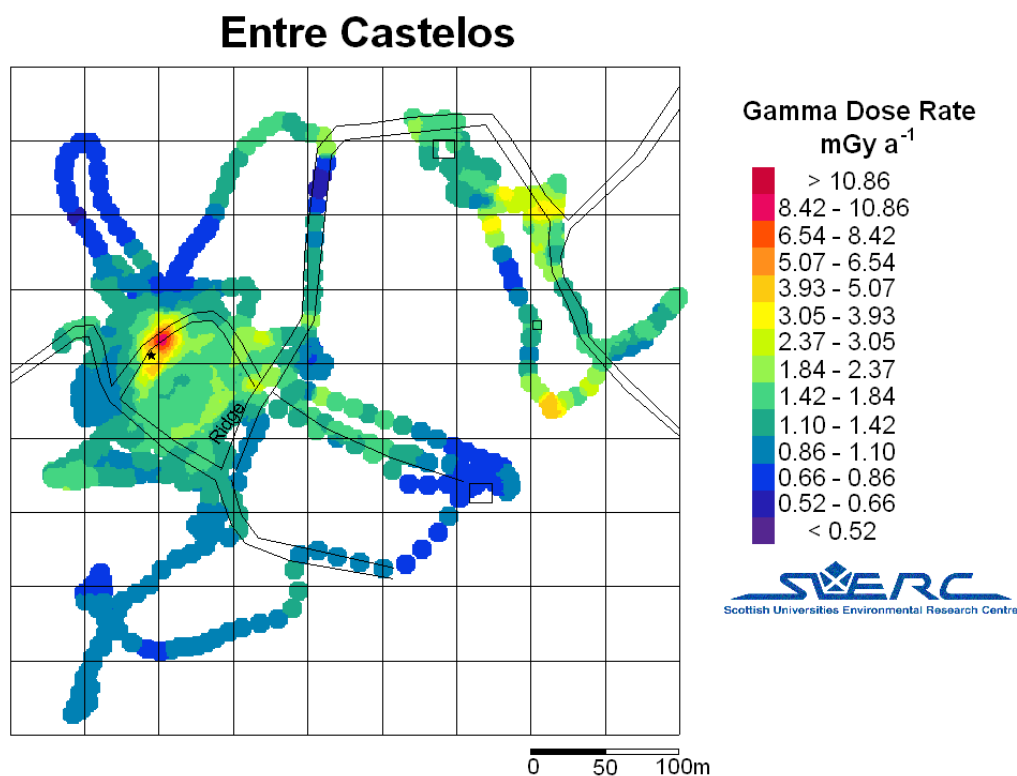
Figure 7: Dose rate distribution at Entre Castelos.
