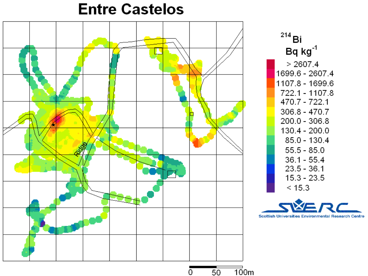
Figure 8: ^{214}\text{Bi} specific activity distribution at Entre Castelos.
