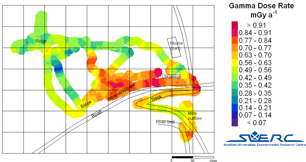
Figure 6: Dose rate distribution around Minas de Massueime.
