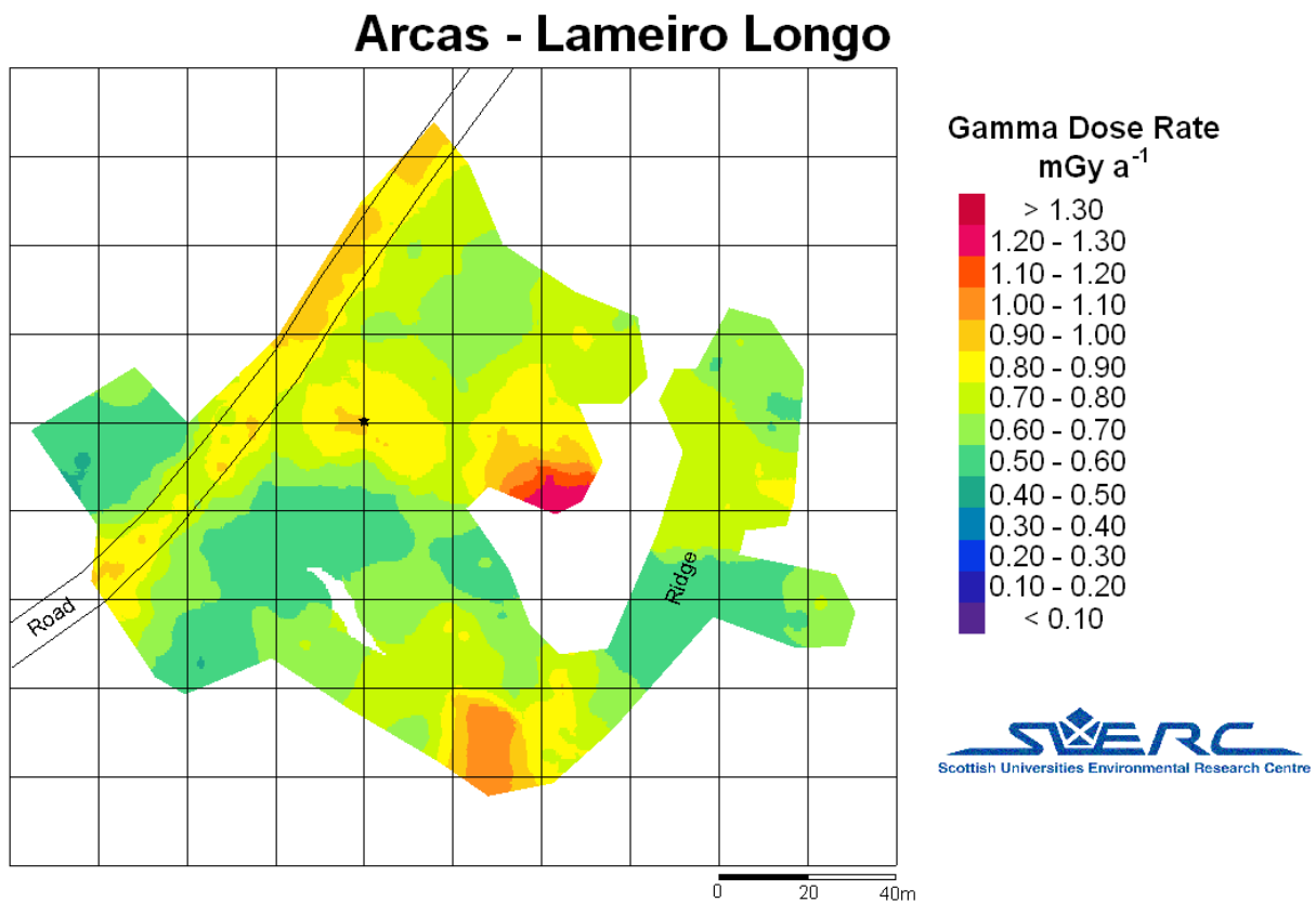
Figure 3: Dose rate distribution at Arcas – Lameiro Longo.
