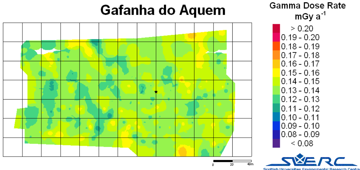
Figure 5: Dose rate distribution at Gafanha do Aquém.
