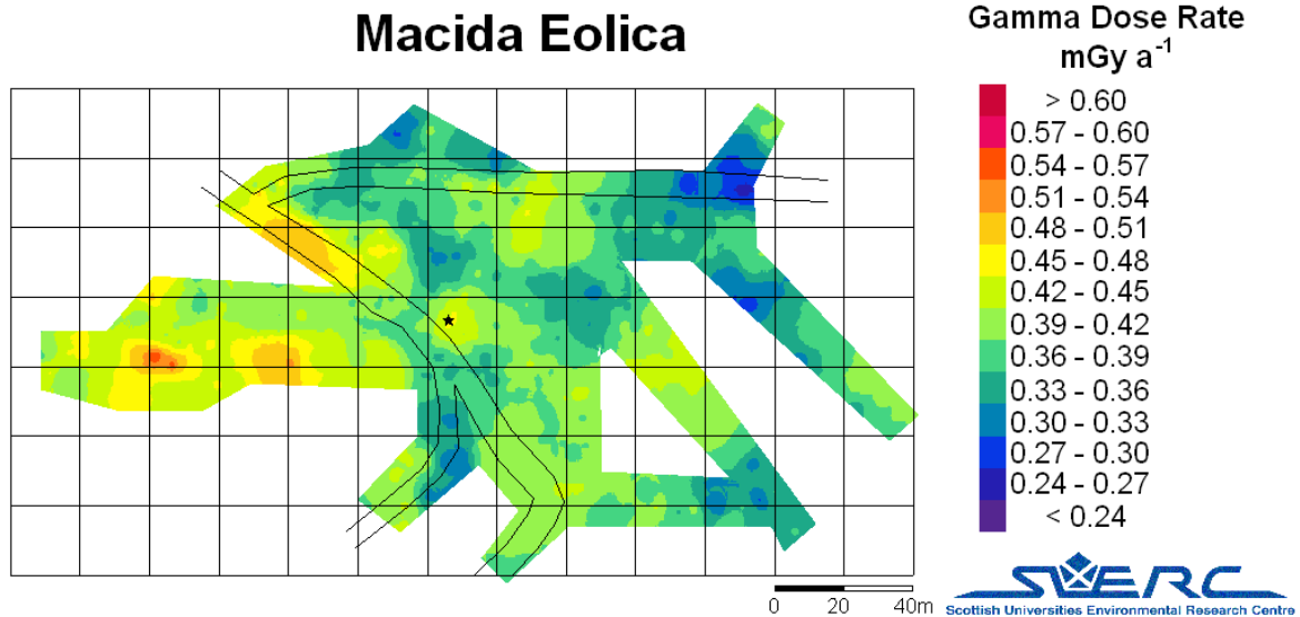
Figure 4: Dose rate distribution at Macida Eólica.
