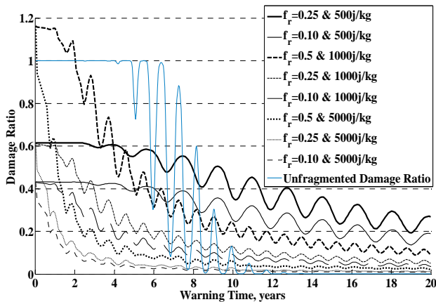
Fig. 17: Damage ratios for a collisional energy of 500 j/kg with disruption levels at f_r=0.25 and f_r=0.1 , and collisional energies of 1000 j/kg and 5000 j/kg with disruption levels at f_r=0.5 , f_r=0.25 and f_r=0.1 .
