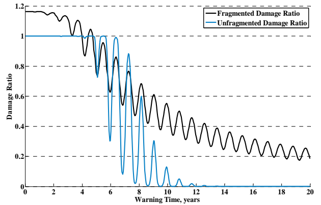
Fig. 16: Damage ratios of Apophis : fragmented case (black line) and unfragmented case (blue line) with 25% error in the delta-velocity.
