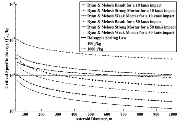
Fig. 1: Critical Specific Energy Q^* to barely catastrophically disrupt an asteroids with a diameter ranging from 40m to 1km using Ryan and Melosh [3] and Holsapple [12]. Ryan and Melosh [3] work provide a scaling law that takes into account both velocity of the impactor and impacted object diameter, while Holsapple [12]'s scaling law is only function of the impacted object diameter.
