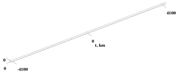
Fig. 9: \sim 97\% probability volume for a fragment with mass 10^{10}\text{kg} at true anomaly of 360^\circ .
