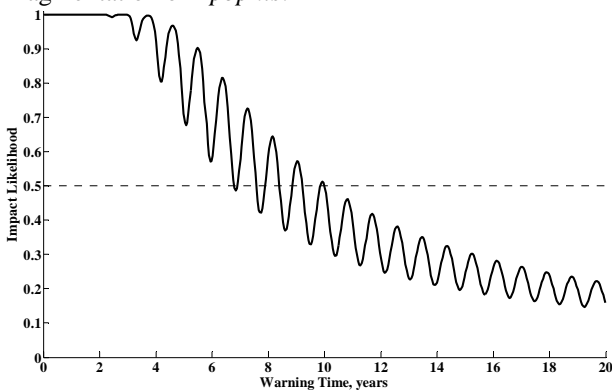
Fig. 12: Impact likelihood for Apophis 's 10^{10} kg-fragments as a function of warning time or time span between break-up and impact. The integrated volume is a sphere of radius 2.16R_{\oplus} with centre at the position of the unperturbed Apophis (Table 1) at time t_{MOID} . Break up is triggered by an m_{s/c} of 10,000kg providing 500 j/kg of SKE, which in turn provides a mean velocity \mu \sim [0.02m/s \ 0 \ 0] and a standard deviation \sigma \sim [0.013 \ 0.013 \ 0.013]m/s to the 10^{10} kg-fragments.
