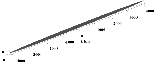
Fig. 8: \sim 97\% probability volume for a fragment with mass 10^{10}\text{kg} at true anomaly of 315^\circ .
