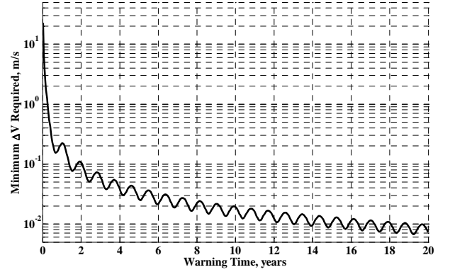
Fig. 2: Minimum Change of velocity to deviate Apophis by a distance 2.16 \times R_{\oplus} as a function of warning time. Warning time is referred here as the time available to correct the trajectory of a threatening object, thus the time difference between the instant at which the change of velocity takes place and the time of the hypothetical impact.
