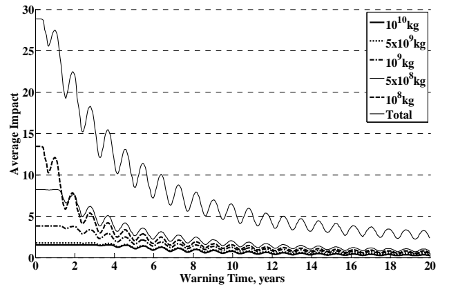
Fig. 15: Average number of impacts for each fragment size group.
