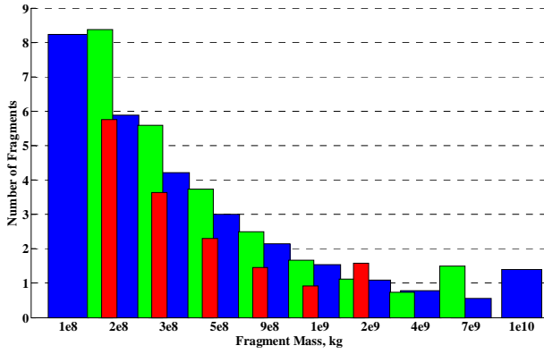
Fig. 13: Approximated number of pieces expected to be found in a fragmentation cloud of an asteroid with 2.7 \times 10^{10} kg of mass resulting from disruptions with f_r=0.5 (blue bars), f_r=0.25 (green bars) and f_r=0.1 (red bars). The largest fragment, i.e., surviving mass of the asteroid, is counted in the initial bin of the histogram for each level of disruption.
