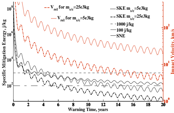
Fig. 3: Minimum specific kinetic energy (SKE) and specific absorbed nuclear energy (SNE) for a mitigation mission at a variable warning time (left Y axis). Relative impact velocities for two kinetic impactors (right Y axis), m_{s/c}=5000\text{kg} and m_{s/c}=25000\text{kg} . The enhancement factor is assumed 2 as a conservative value for this computation [8].
