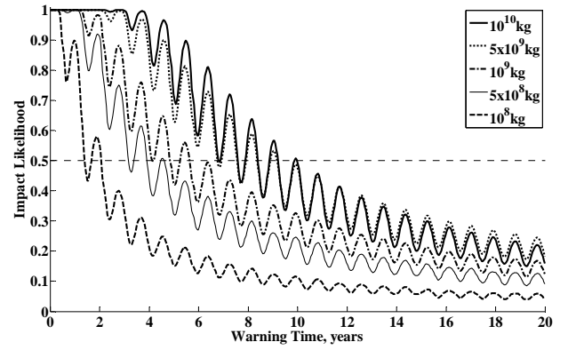
Fig. 14: Impact likelihood evolutions of the 5 fragments size computed.
