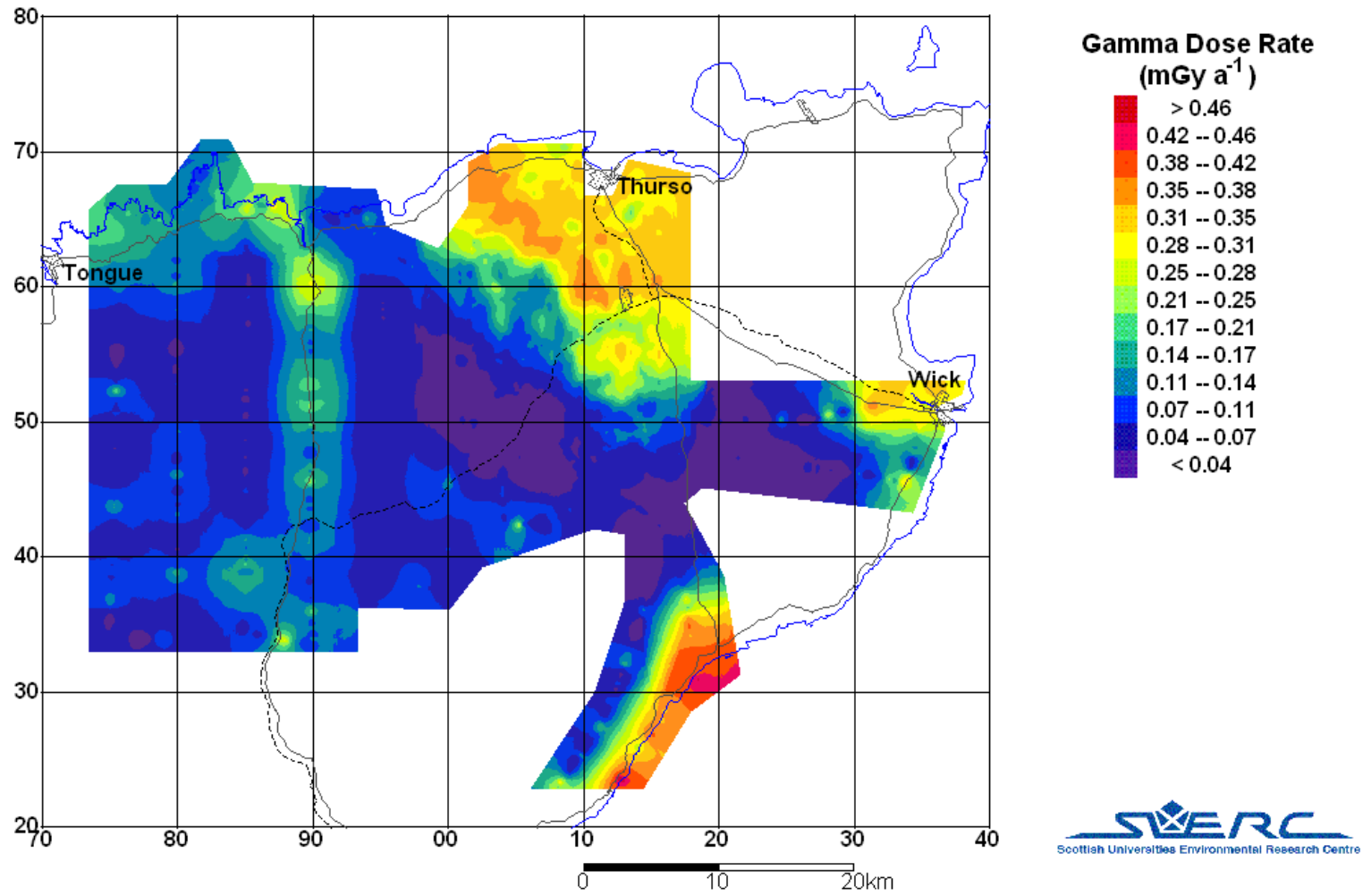
Figure 4.5: Gamma Dose Rate distribution in the Caithness region.
