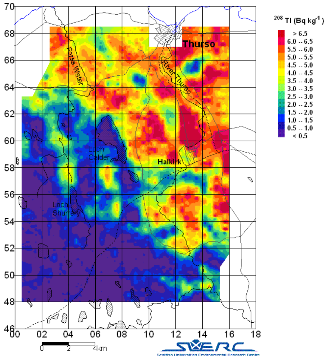
Figure 4.9: ^{208}\text{Tl} distribution in the area around Forss Water and the Thurso River.
