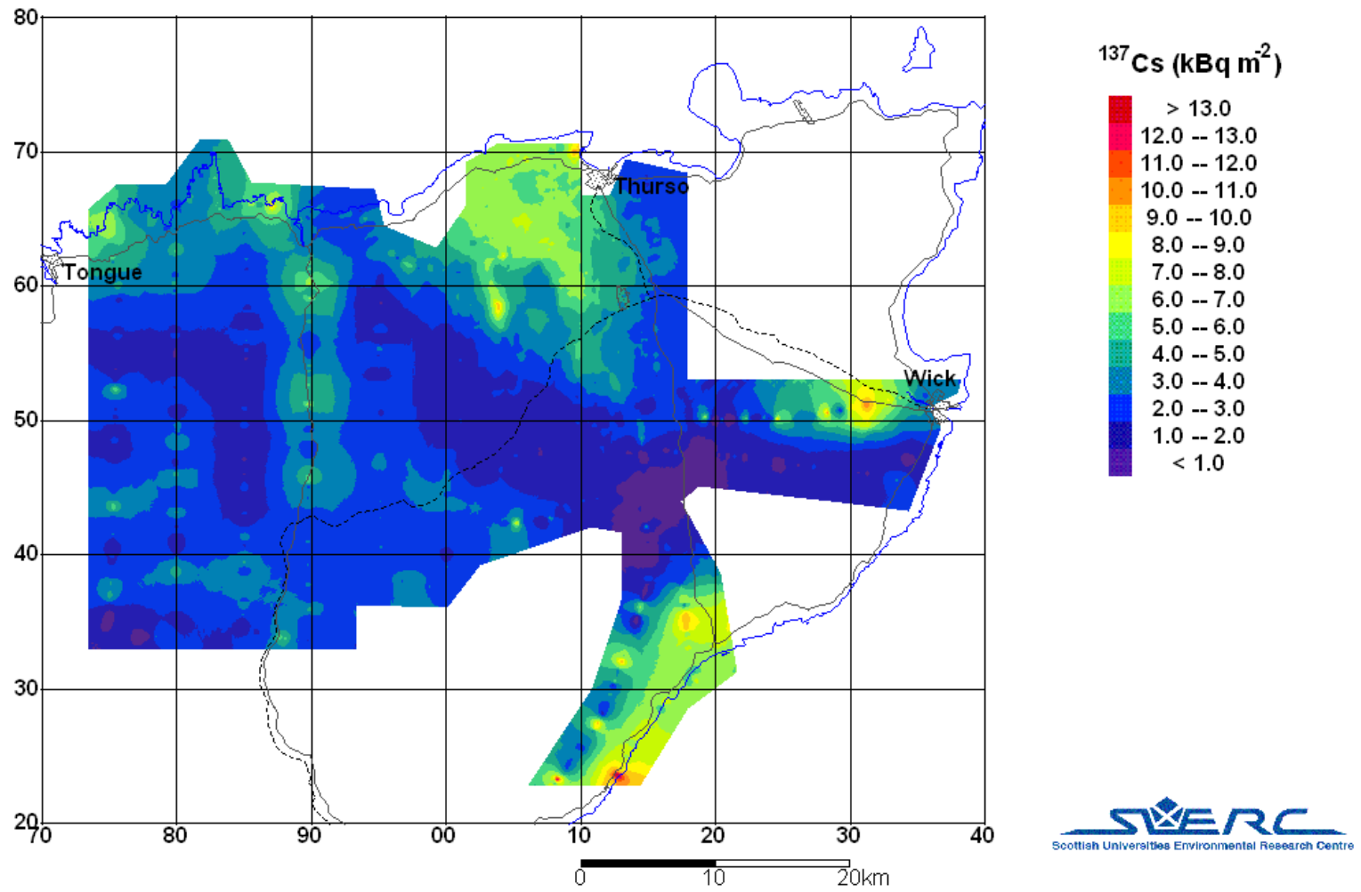
Figure 4.1: ^{137}\text{Cs} distribution in the Caithness region.
