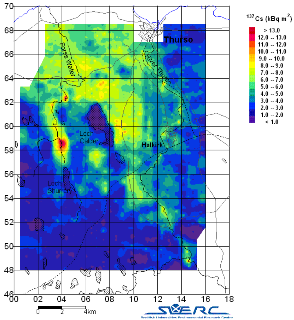
Figure 4.6: ^{137}\text{Cs} distribution in the area around Forss Water and the Thurso River.
