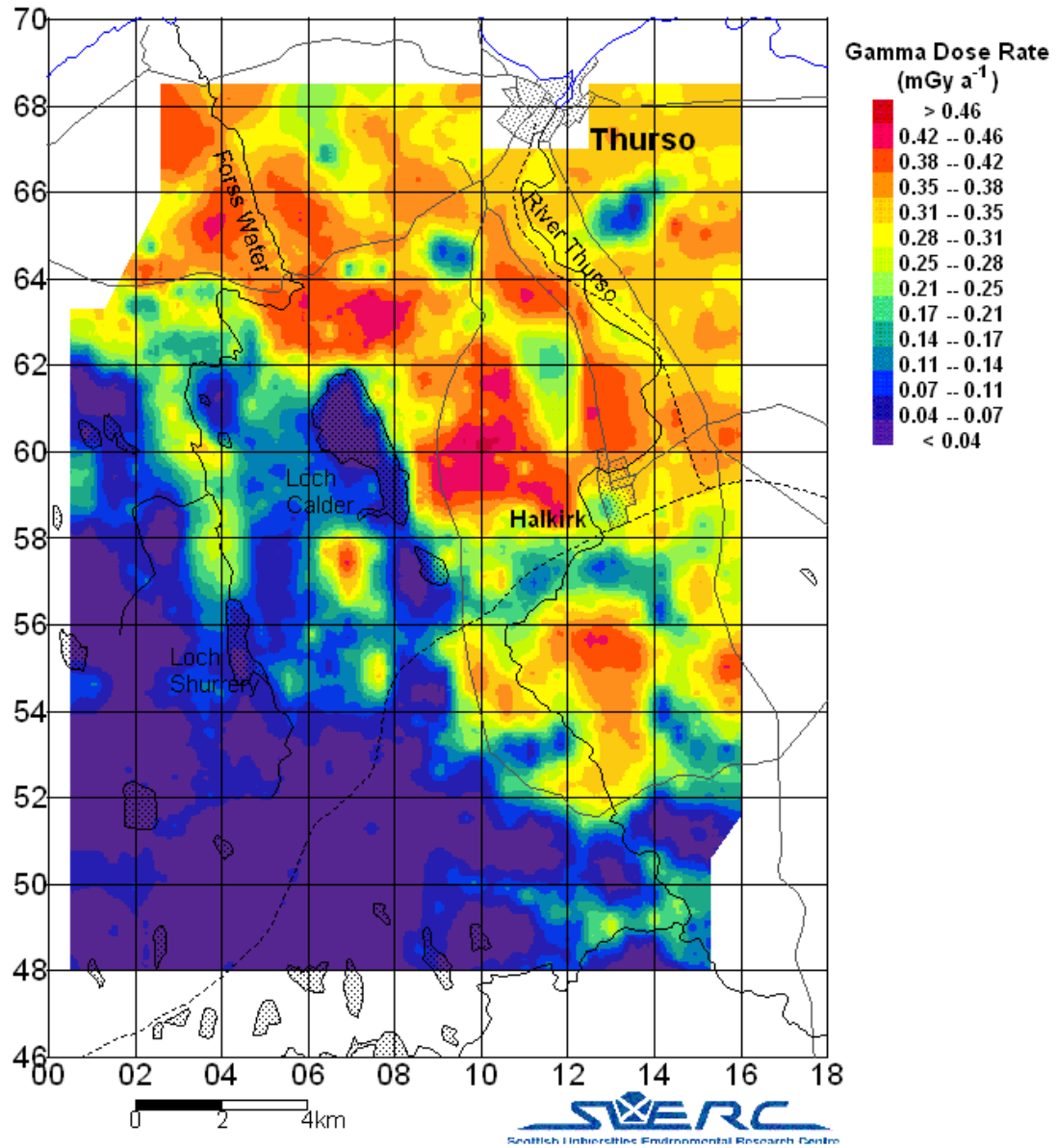
Figure 4.10: Gamma Dose Rate distribution in the area around Forss Water and the Thurso River.
