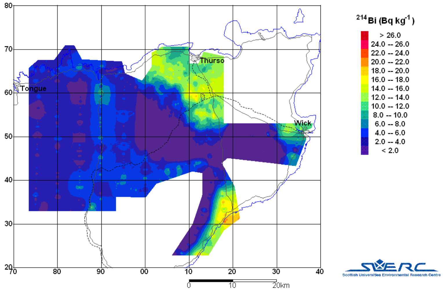
Figure 4.3: ^{214}\text{Bi} distribution in the Caithness region.
