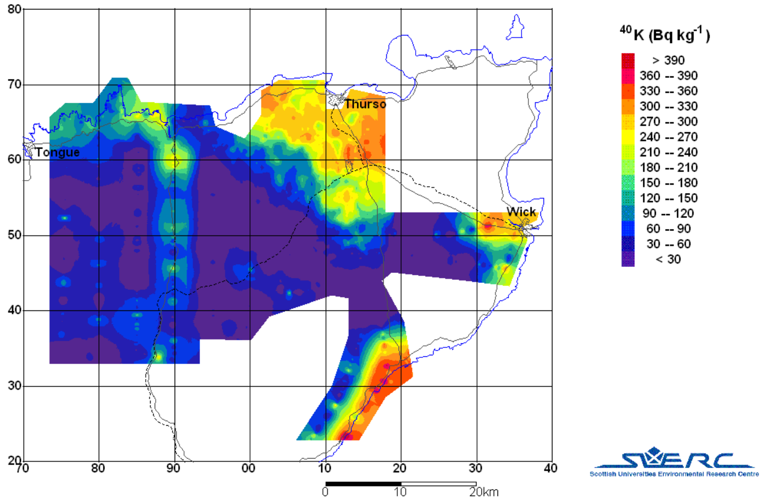
Figure 4.2: ^{40}\text{K} distribution in the Caithness region.
