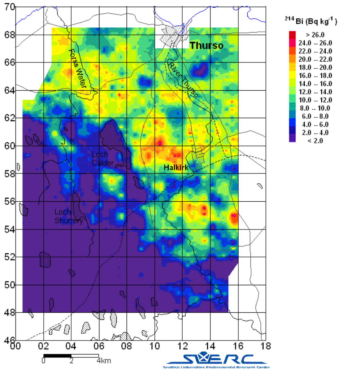
Figure 4.8: ^{214}\text{Bi} distribution in the area around Forss Water and the Thurso River.
