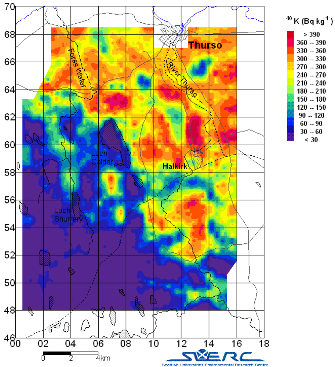
Figure 4.7: ^{40}\text{K} distribution in the area around Forss Water and the Thurso River.
