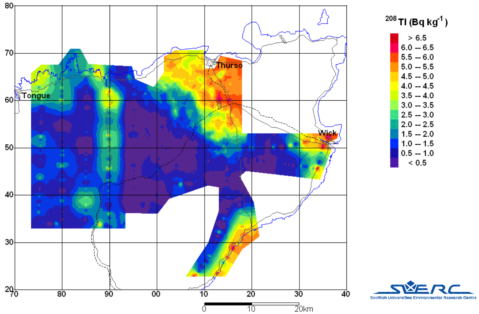
Figure 4.4: ^{208}\text{Tl} distribution in the Caithness region.
