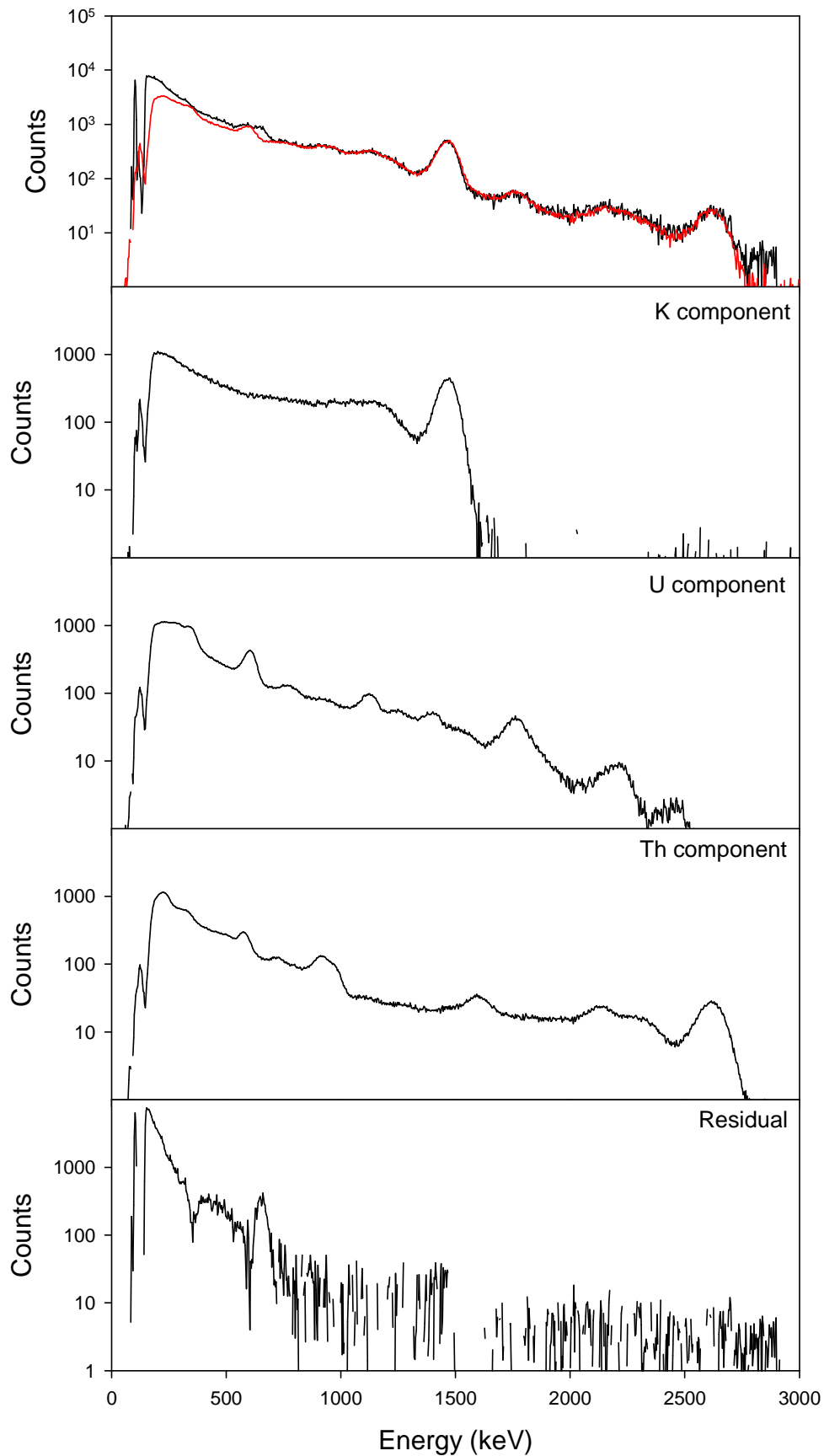
Figure 3.1: Measured spectrum from the field at DERC with the natural series components determined by least squares fitting above 1 MeV, the resulting fitted spectrum (in red) and residual spectrum.
