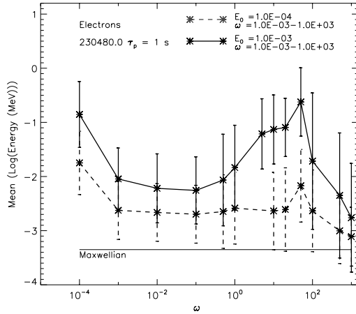
Fig. 7. Mean energy and standard deviation of electron distributions for two amplitudes of the electric field ( E_0 = 0.001, 0.0001 ) and for range of frequencies. The mean energy of the initial Maxwellian distribution is shown as a straight full line. The constant electric field case is represented in \omega = 0.001 .
