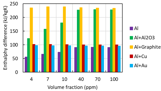
Figure 4. Storage capacities of nanoparticles
