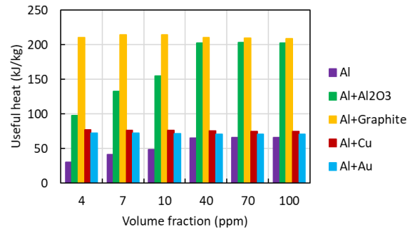
Figure 3. Useful heat capacities of nanoparticles
