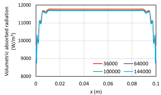
Figure 2. This shows that small differences have been obtained and can be neglected after mesh number of 64000.
