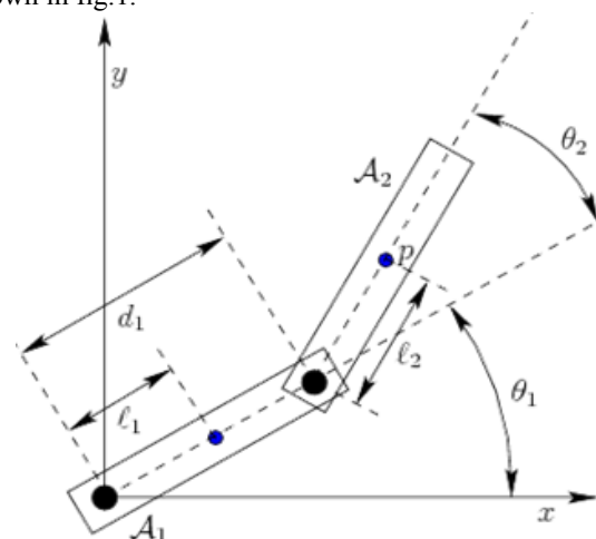
Fig. 1 Representation of 2-DOF robotic manipulator
