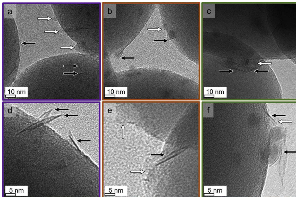
Fig. 3. Transmission electron micrographs of spent and passivated model catalysts (a) CAT A1, (b) CAT B1, as well as (c) CAT C and (d–e) enlarged images of needle-like structures (demarcated with black arrows) on top of nanoparticles surrounded by a cloud of material with different density (demarcated with white arrows).
