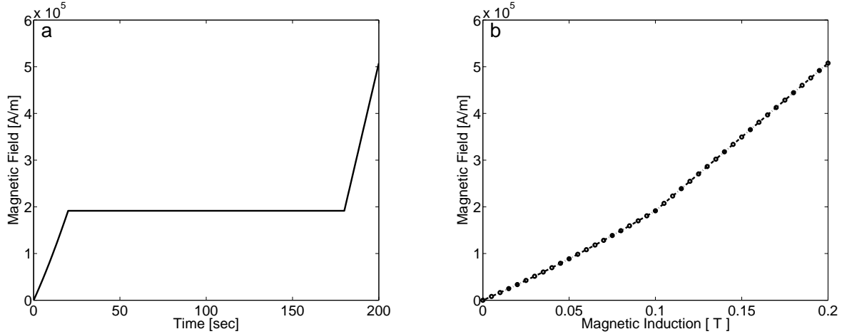
Figure 6: Magneto-elastic curing model with the three phase magnetic loading: (a) Magnetic field over curing time (b) Magnetic field vs magnetic induction that highlights stiffness gain under chain cross-linking where the magnetic stress response is higher in the second loading phase compared to the first one due to stiffness gain in the longer holding period (21-180 sec)
