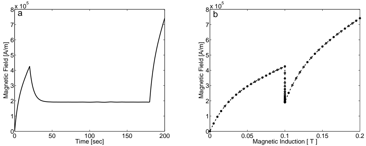
Figure 9: Magneto-viscoelastic curing model with the three phase magnetic loading : (a) Magnetic field over curing time with a quick relaxation phenomenon in the holding phase (b) Magnetic field vs magnetic induction that highlights a stiffness gain due to the chain cross-linking where a kink during holding time indicates magnetic field/stress relaxation
