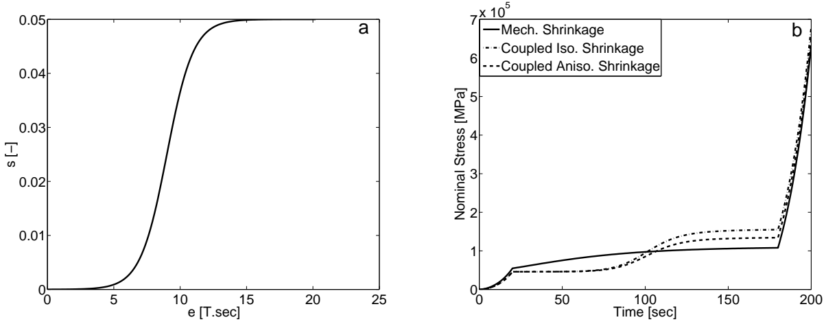
Figure 16: Magnetic-load-dependent shrinkage model: (a) Degree of exposure e results from the three-phase magnetic load (b) Magnetic-induction-dependent shrinkage-generated stress responses for the three-phase magneto-mechanical load
