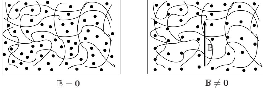
Figure 17: Particles alignment during curing: I) In the absence of a magnetic load, isotropic material; II) Preferred direction in the presence of a magnetic field
