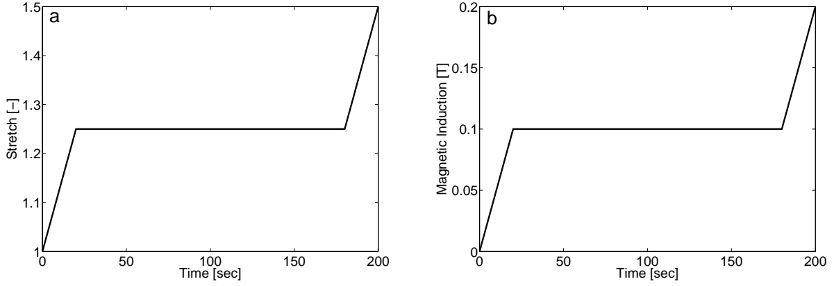
Figure 4: Three-phase loading, i.e. pull-hold-pull : (a) Mechanical stretch over curing time (b) Magnetic induction over curing time
