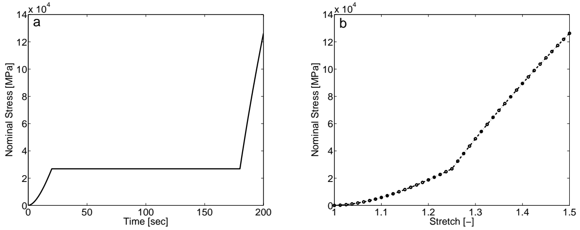
Figure 5: Magneto-elastic curing model with the three phase mechanical loading: (a) Mechanical stress over curing time (b) Mechanical stress vs stretch that highlights stiffness gain. The stress response is higher in the second loading phase compared to the first one due to stiffness gain in the longer holding period (21-180 sec)
