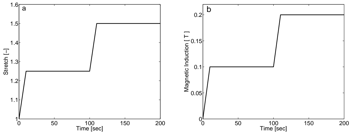
Figure 10: Four-phase loading : (a) Mechanical stretch over curing time, (b) Magnetic induction over curing time
