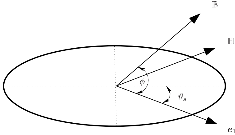
Figure 13: An ellipse illustrates the principal directions of total Cauchy stress \sigma as its axes while respective alignments of magnetic induction \mathbb{B} , magnetic field \mathbb{H} and Cartesian direction e_1
