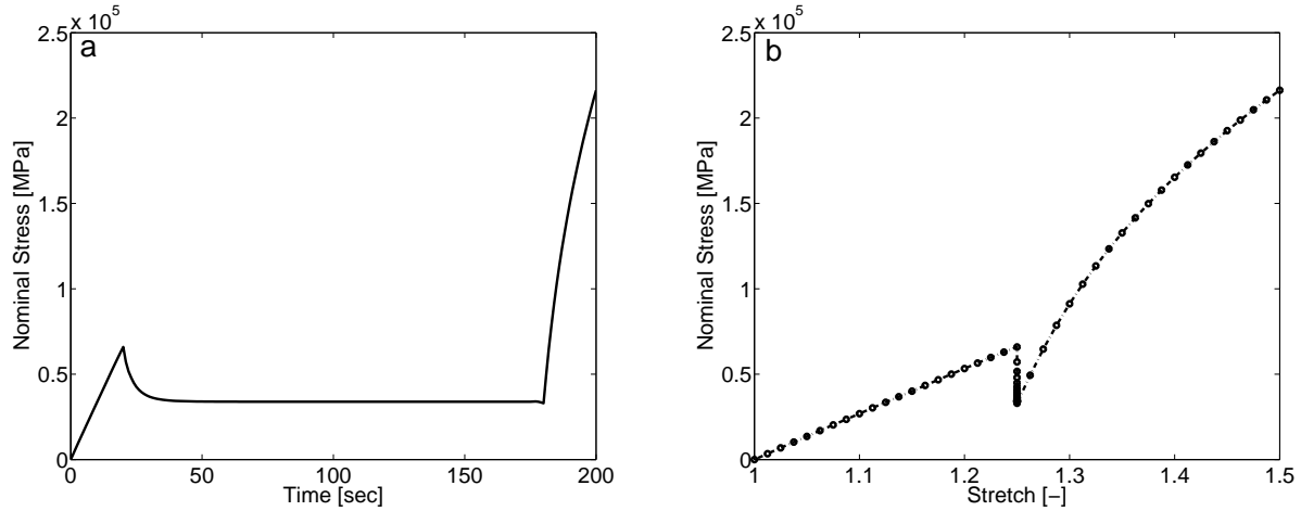
Figure 7: Magneto-viscoelastic curing model with the three phase mechanical loading : (a) Mechanical stress over curing time (b) Mechanical stress vs stretch with a stress relaxation during holding time. The mechanical stress response is higher in the second loading phase compared to the first one due to stiffness gain in the longer holding period
