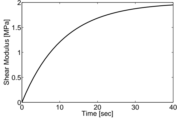
Figure 3: Evolution of the shear modulus \mu(t) with [\mu_{in}, \mu_\infty, \kappa_\mu] = [0.0001 \text{ N/mm}^2, 2.0 \text{ N/mm}^2, 0.0925 \text{ s}^{-1}]
