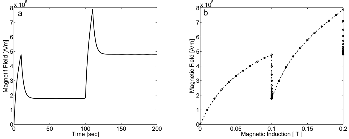
Figure 12: Magneto-viscoelastic curing model with the pull-hold-pull-hold magnetic loading: (a) Magnetic field over curing time (b) Magnetic field vs magnetic induction that highlights stiffness gain due to a continuous chain crosslinking. However, the stress relaxation in the two holding phases are the same due to a constant value of the magnetic relaxation parameter, T_m
