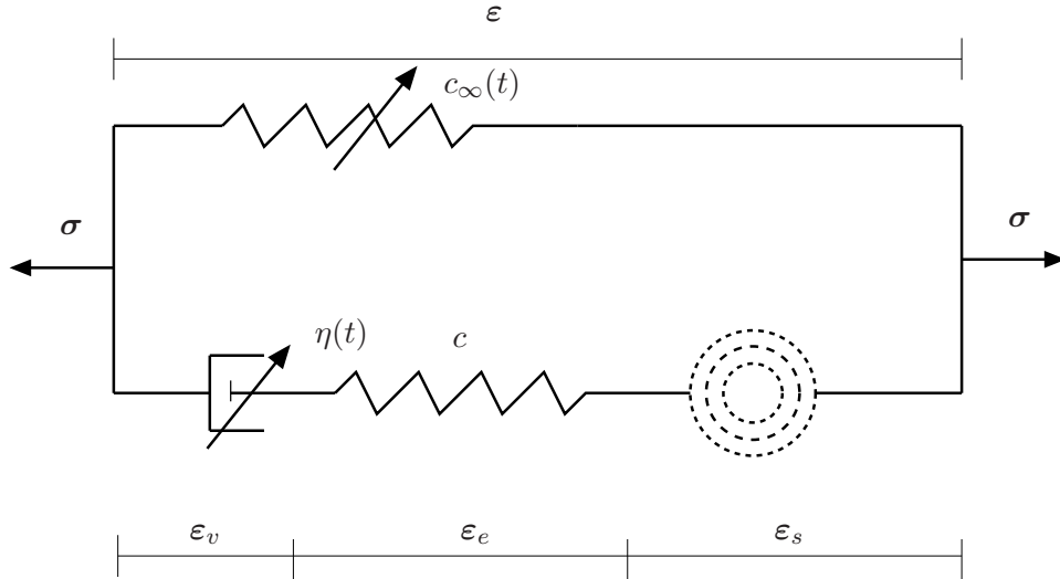
Figure 1: One-dimensional cure-dependent mechanical viscoelastic model with a shrinkage element of deformation \epsilon_s . It mimics the idea of a Zener-type viscoelastic standard solid model with a time-dependent spring, a time-dependent dash-pot and a time-dependent shrinkage-induced fictitious element connected in parallel
