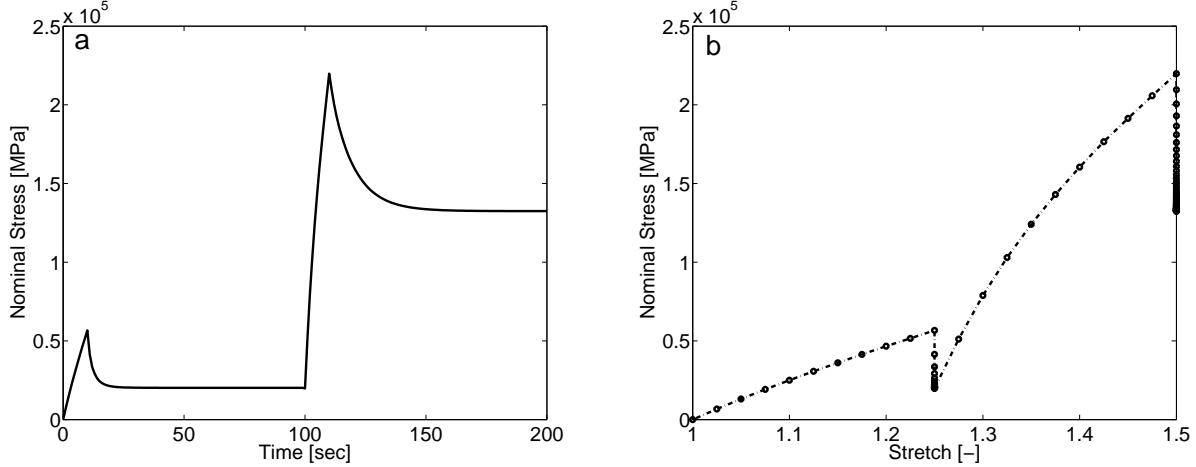
Figure 11: Magneto-viscoelastic curing model with the four phase mechanical loading : (a) Purely mechanical stress over curing time as produced from a four-phase purely mechanical loading (b) Purely mechanical stress vs stretch that highlights stiffness gain in successive loading phases. The stress relaxation is decelerated in the second holding phase due to a time-evolving characteristics of the mechanical relaxation parameter, T_v
