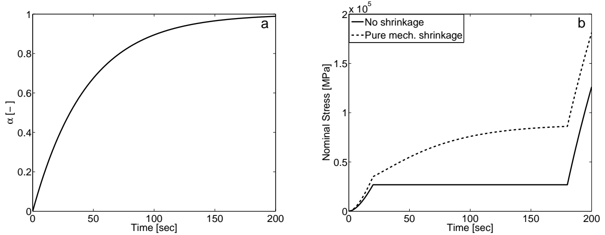
Figure 15: Shrinkage-induced stress development under a three phase mechanical loading: (a) Degree of cure using an exponential saturation function (b) Shrinkage-induced stress responses for the three-phase purely mechanical load
