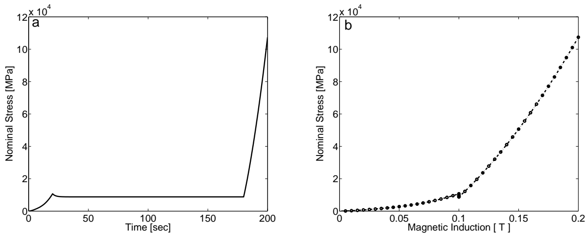
Figure 8: Magneto-viscoelastic curing model with the three phase magnetic loading: (a) Mechanical stress over curing time demonstrating a small but quick mechanical stress relaxation (b) Mechanical stress over magnetic induction that highlights a stiffness gain under chain cross-linking where a kink during holding time indicates mechanical stress relaxation
