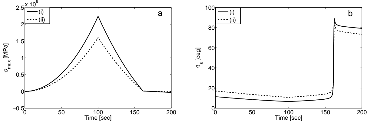
Figure 14: (a) Maximum principal Cauchy stress \sigma_{\max} with time ; (i) \phi = \pi/6 and (ii) \phi = \pi/4 . (b) Evolution of the orientation angle \vartheta_s ; (i) \phi = \pi/6 and (ii) \phi = \pi/4
