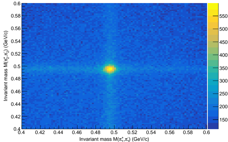
Figure 4. Correlation between the invariant mass of one \pi^+\pi^- pair and the other \pi^+\pi^- pair. The spot at the center shows the situation where both pion pairs come from decays of two K_S^0 .
