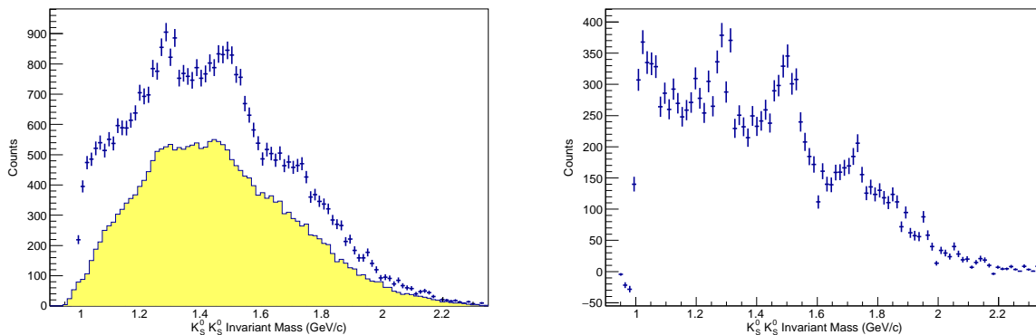
Figure 5. The left histogram with the error bars shows the signal + background, whereas the shaded (yellow online) histogram is the average sideband background. The right histogram is the sideband subtracted histogram. The peak near 1.50 GeV is the region of interest.
