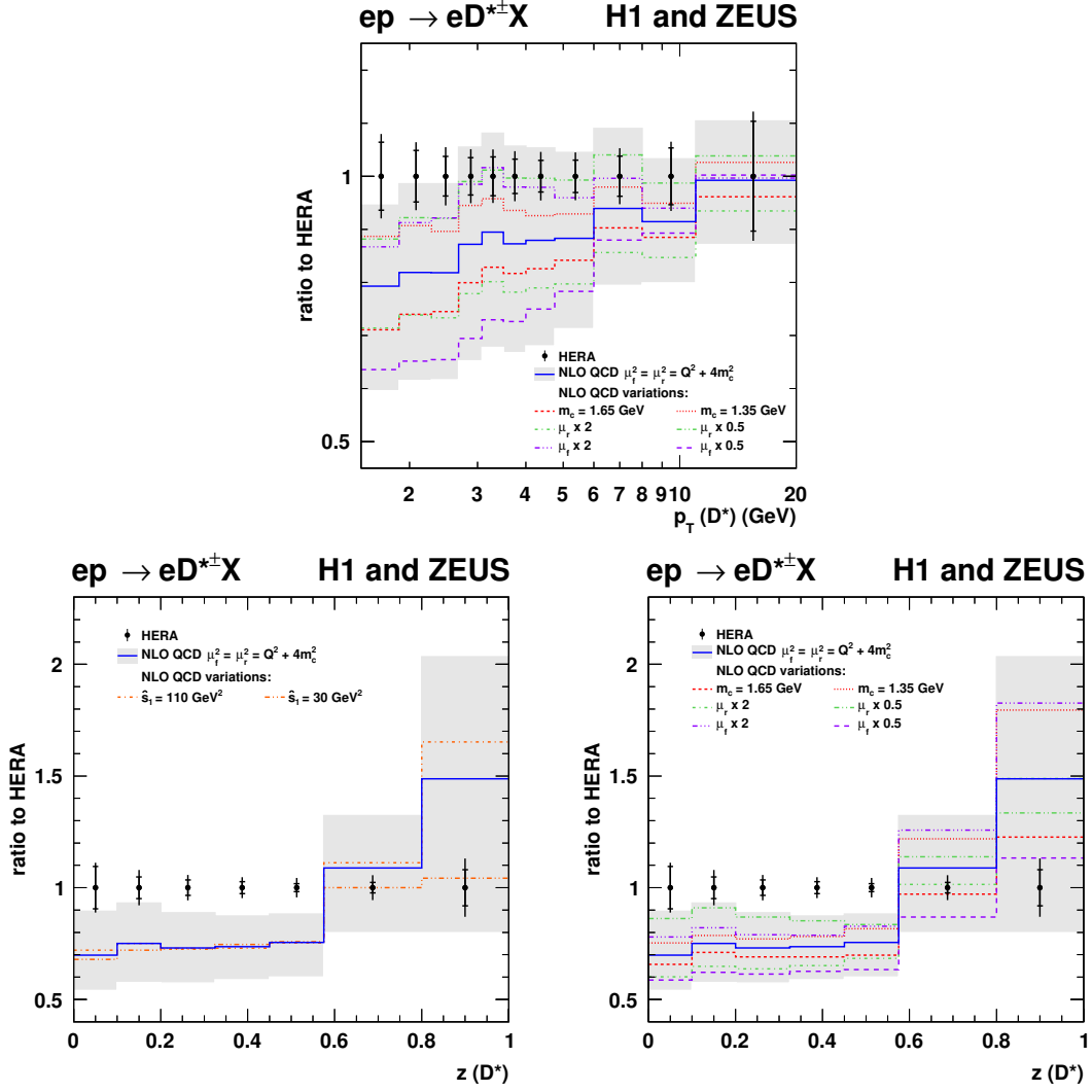
Figure 11. Differential D^{*\pm} -production cross section (ratio to data) as a function of p_T(D^*) (top) and z(D^*) (bottom) compared to NLO predictions with different variations: charm-quark mass m_c , renormalisation scale \mu_r , factorisation scale \mu_f and fragmentation bin boundary \hat{s}_1 .
