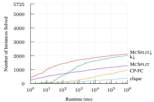
Figure 4: Cumulative numbers of instances solved over time for the maximum common connected subgraph problem on the large subgraph isomorphism benchmark suite.
