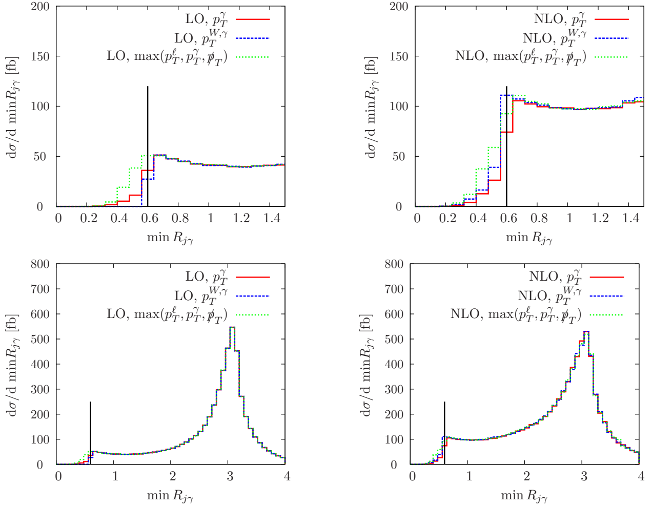
Figure 3: Minimal photon-jet separation in the azimuthal angle – pseudorapidity plane for W^- \gamma +jet production at the LHC. Plotted are the leading order and next-to-leading order distributions for different isolation scales \mathcal{E} = p_T^\gamma, p_T^{W,\gamma}, \max(p_T^\ell, p_T^\gamma, \not{p}_T) in Eq. (13). The upper row displays the lower row’s \min R_{j\gamma} distributions around the isolation cone in more detail. The isolation parameter is \delta_0 = 0.6 (indicated by the vertical line), and \mu_F = \mu_R = 100 GeV. Cuts are chosen as described in the text.
