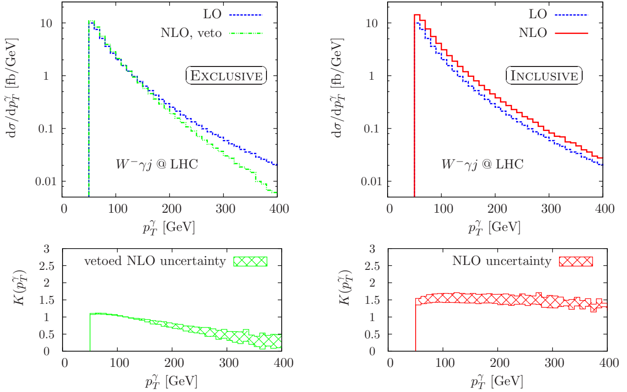
Figure 5: Transverse momentum of the photon for exclusive (left panel) and inclusive W^- \gamma + jet production (right panel). The uncertainty bands refer to fixed scale variations around \mu_R = \mu_F = 100 GeV by a factor two in the NLO computation only.
