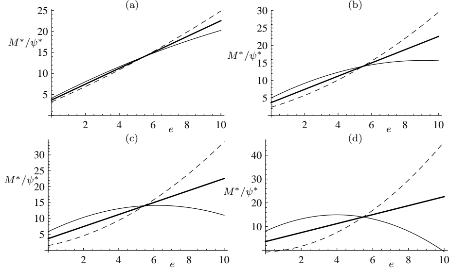
Figure 3: Plots of M^*/\psi^* versus e for \lambda_z = 1 and \eta = 1.7 with the following values of \alpha^* : (a) 1, 0, -1; (b) 3, 0, -3; (c) 5, 0, -5; (d) 10, 0, -10, corresponding in each panel to the continuous, thick continuous and dashed curves, respectively.
